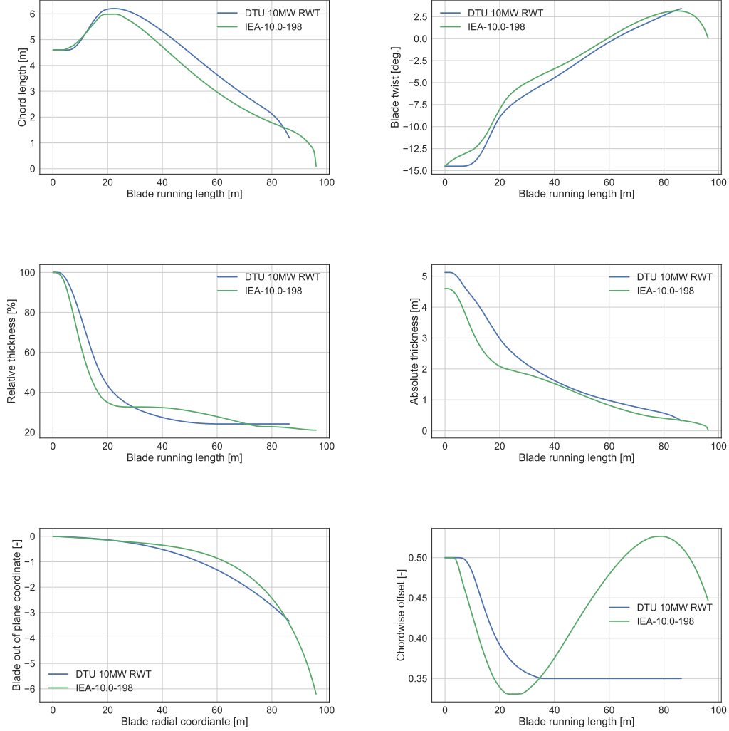
Figure 19: Optimized 10-MW blade planform compared to the baseline DTU 10-MW RWT.
