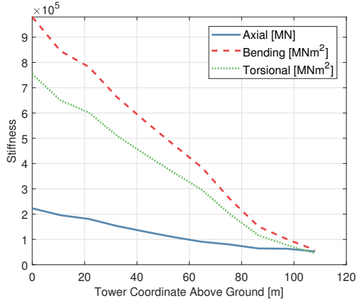
(c) Axial, bending and torsional stiffness distributions
