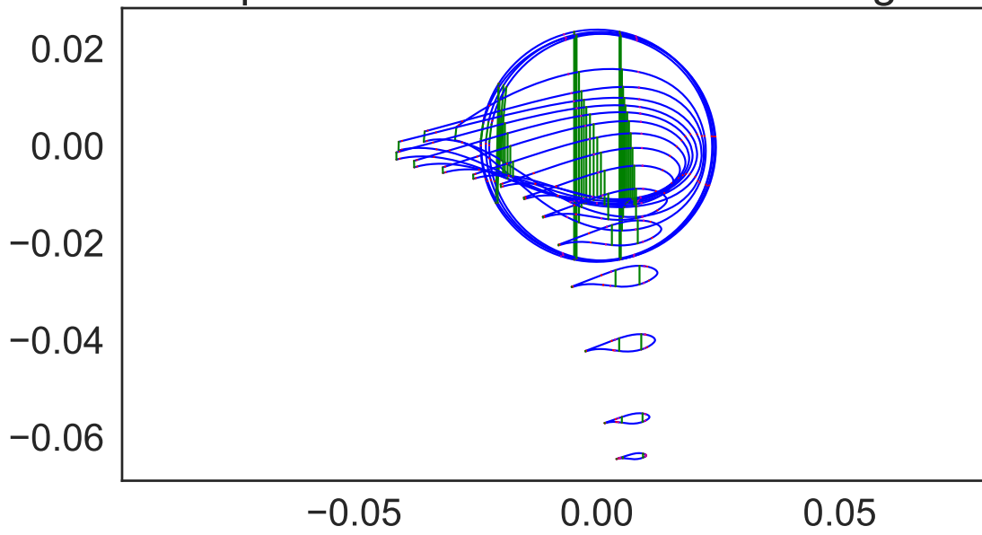
Tip view - mold orientation 6.6 deg.
