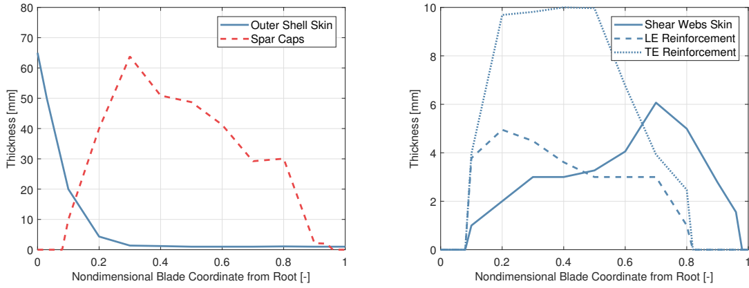
Figure 10: Thicknesses of the structural components of the blade of the land-based wind turbine.
