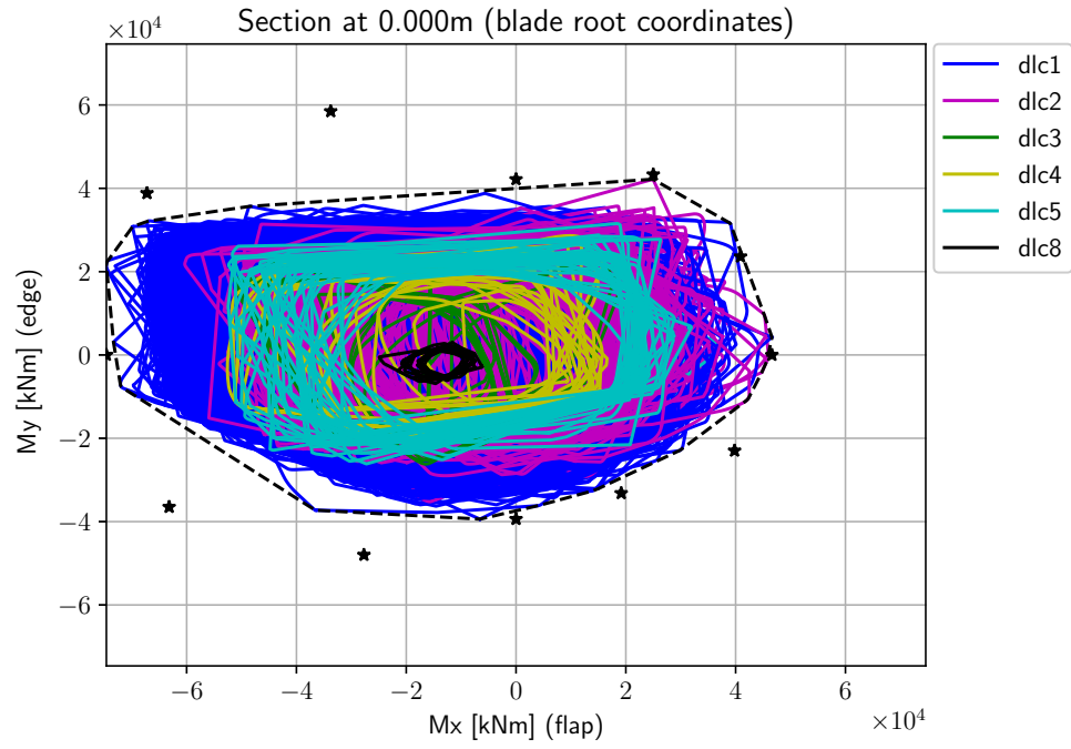
Figure 34: Loads envelope at blade root. Black star refers to the projected load.
