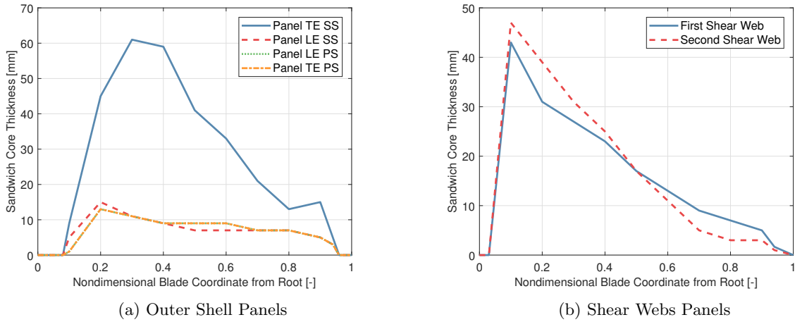
Figure 11: Thicknesses of the core in the sandwich panels of the blade of the land-based wind turbine.
