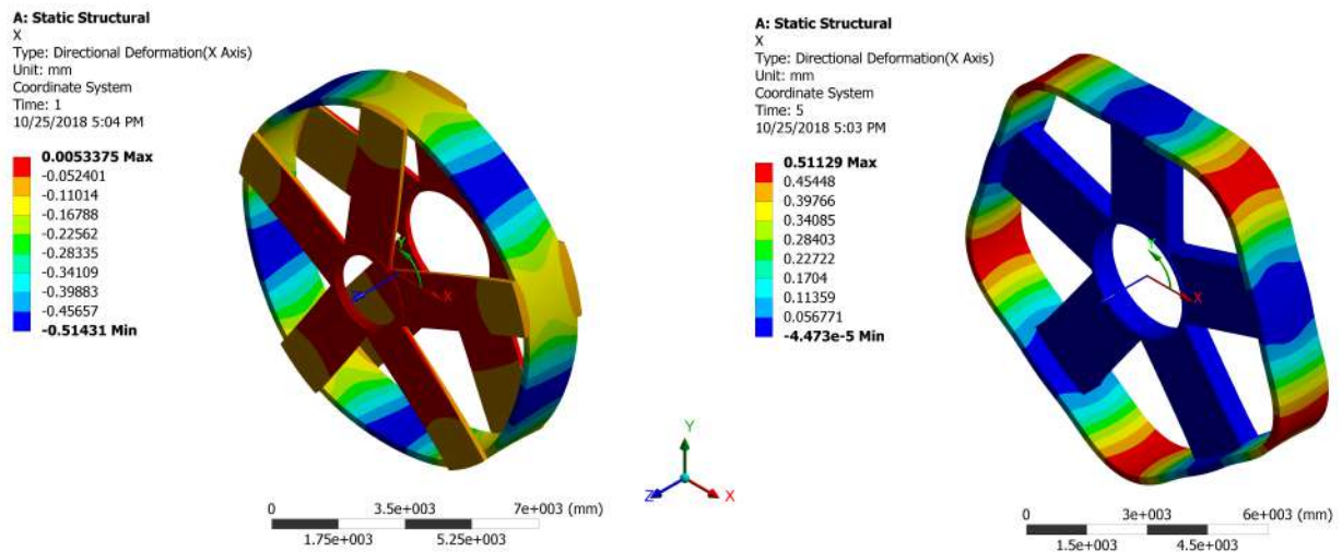
Figure 32: Analysis of the structural design.
