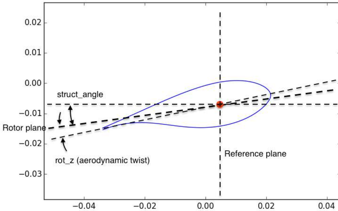
Figure 24: Schematic showing the definition of the structural angle for the 10-MW rotor.
