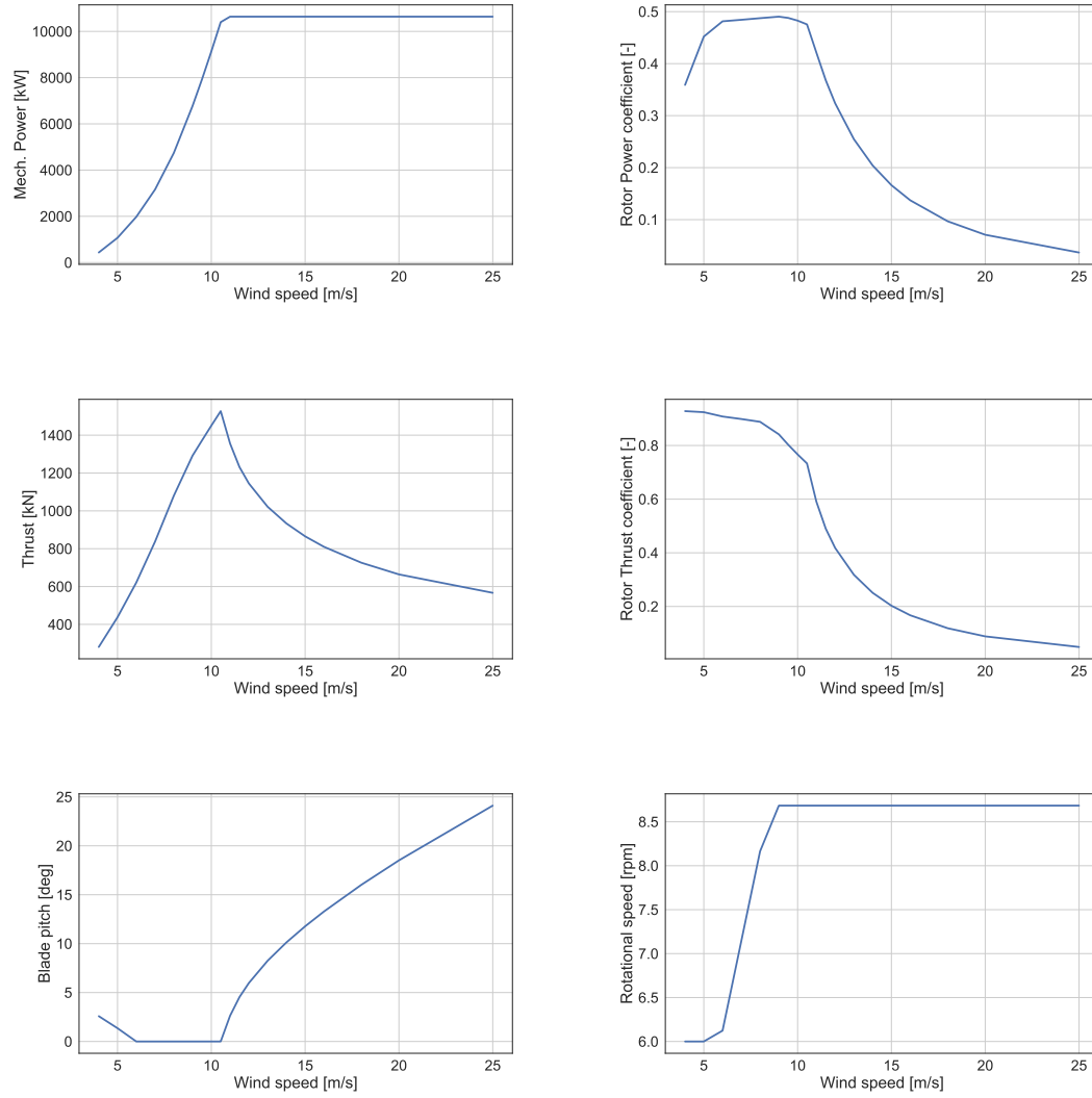
Figure 33: Steady-state performance and operation of the 10-MW rotor.
