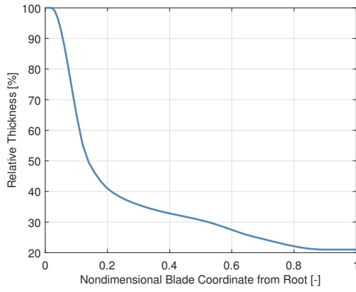
(c) Relative thickness
