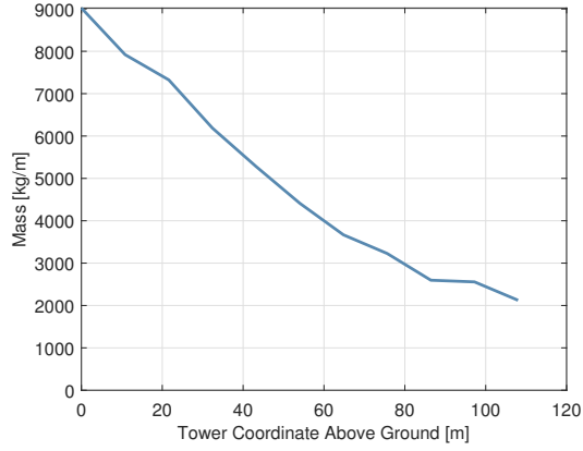
(a) Mass distribution
