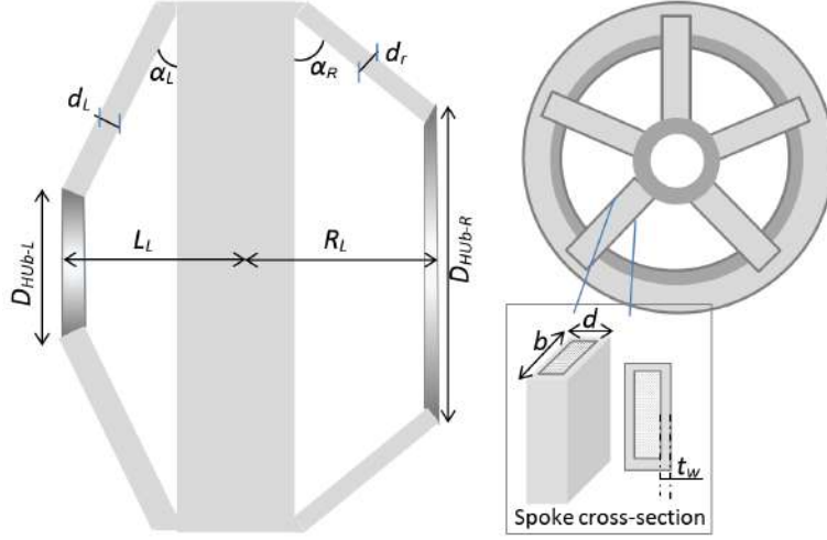
Figure 30: Structural design parameters.
