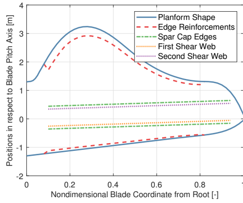
Figure 9: Positions along blade span of the various structural components.
