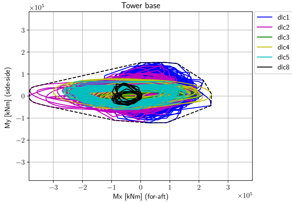
Figure 35: Loads envelope at tower bottom. Black star refers to the projected load.
