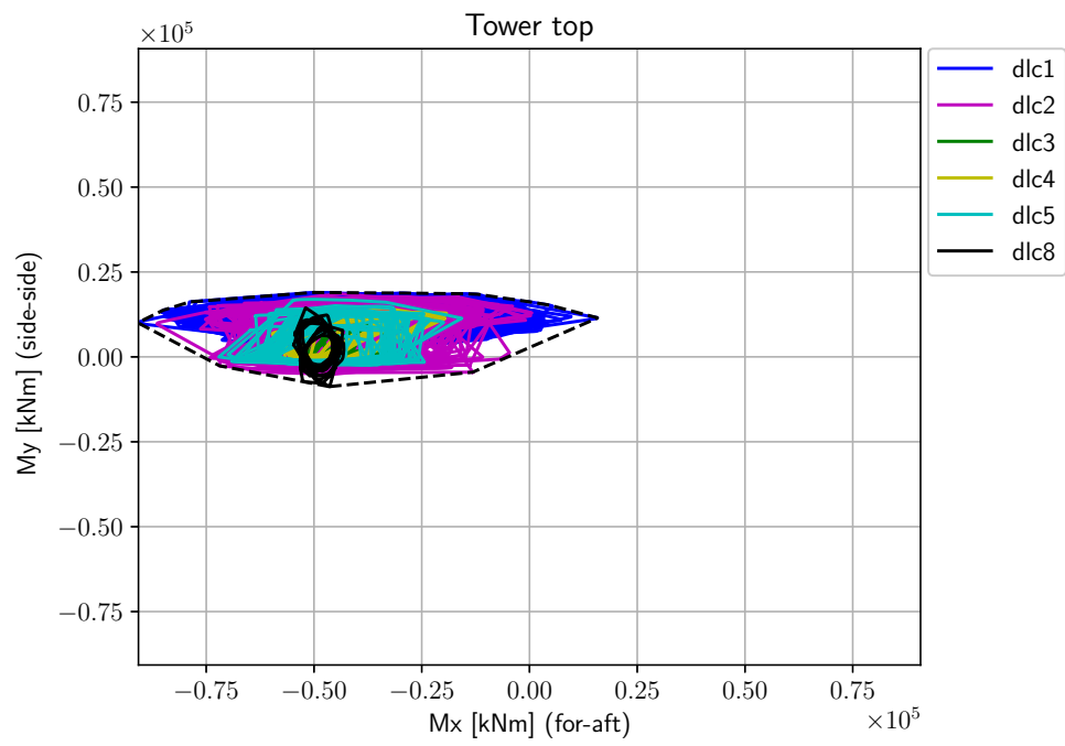
Figure 36: Loads envelope at tower top. Black star refers to the projected load.
