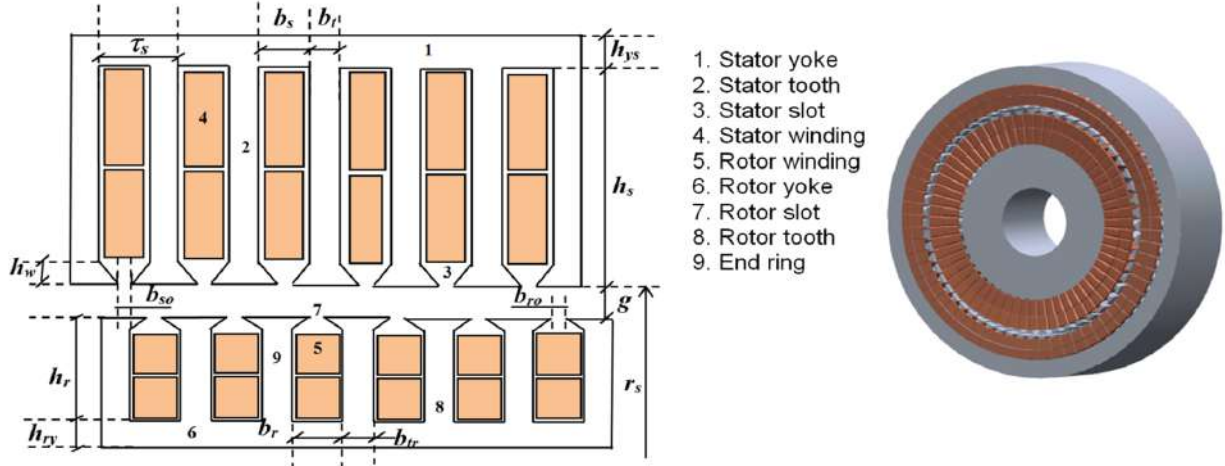
Figure 14: DFIG module within GeneratorSE. Design dimensions and CAD illustration reproduced from [28].
