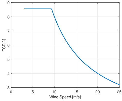
(c) Tip-speed ratio
