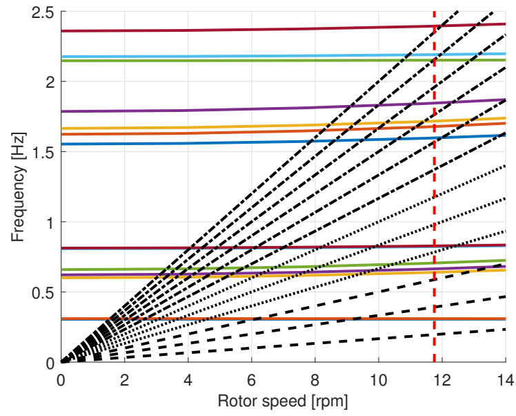
Figure 18: Simplified Campbell diagram for the land-based wind turbine. The horizontal lines represent the modes listed in Table 8.
