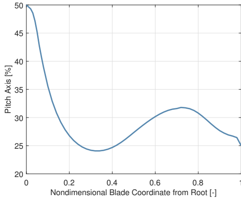
(e) Pitch axis positioning
