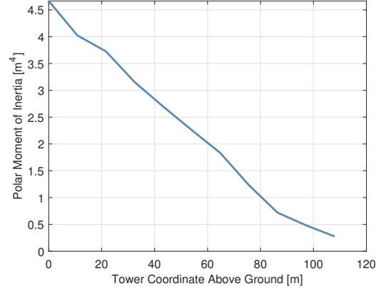
(b) Polar moment of inertia distribution
