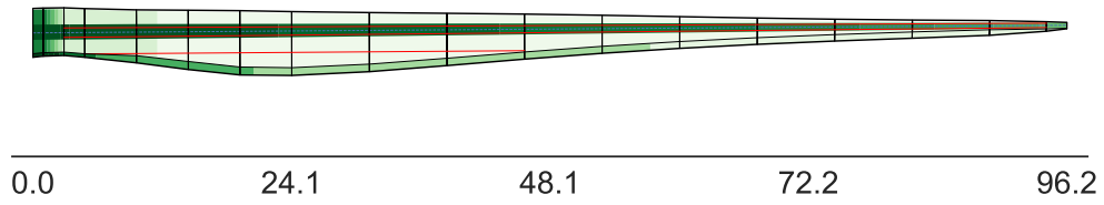
Figure 21: Top view of the 10-MW blade showing internal structural geometry.
