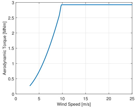
(e) Aerodynamic torque
