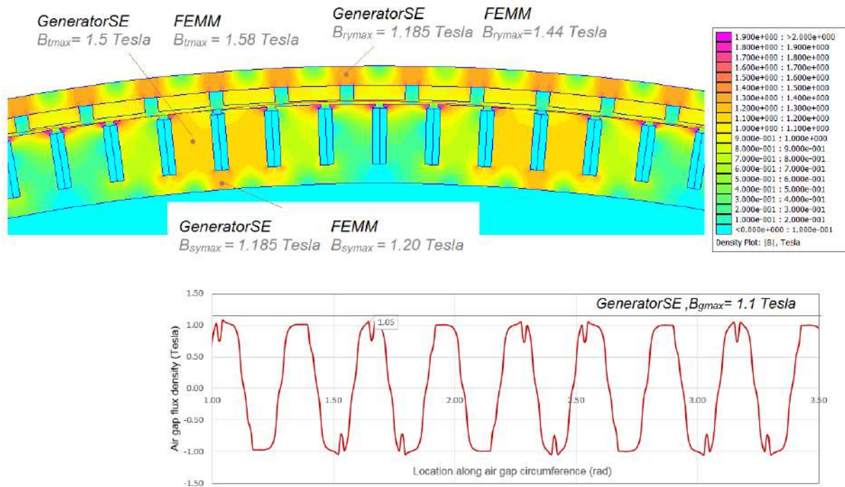
Figure 31: Analysis of the electromagnetic design.
