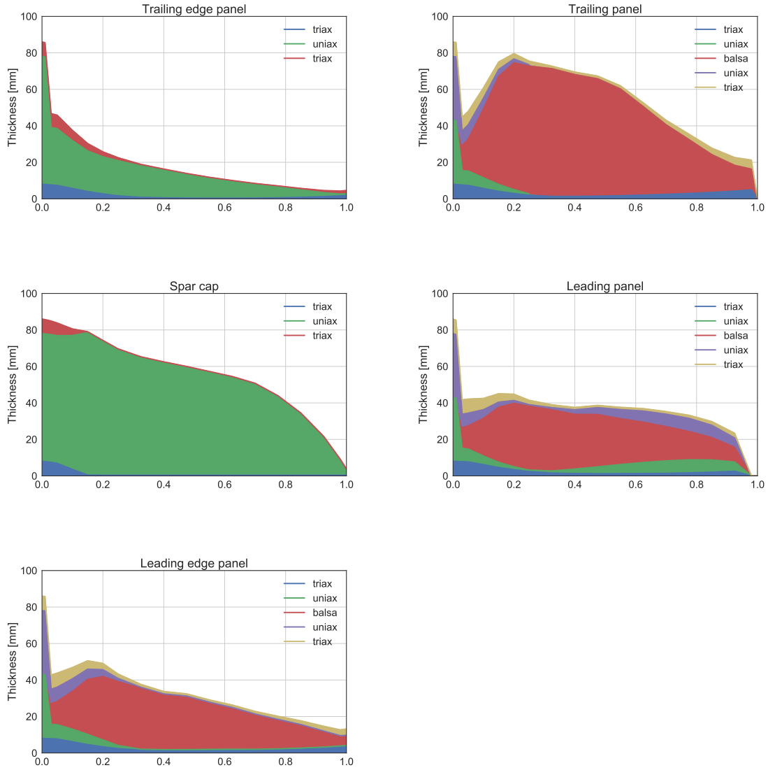
Figure 25: Material stacking sequence for each region along the optimized blade. The x-axis represents the non-dimensional blade span.
