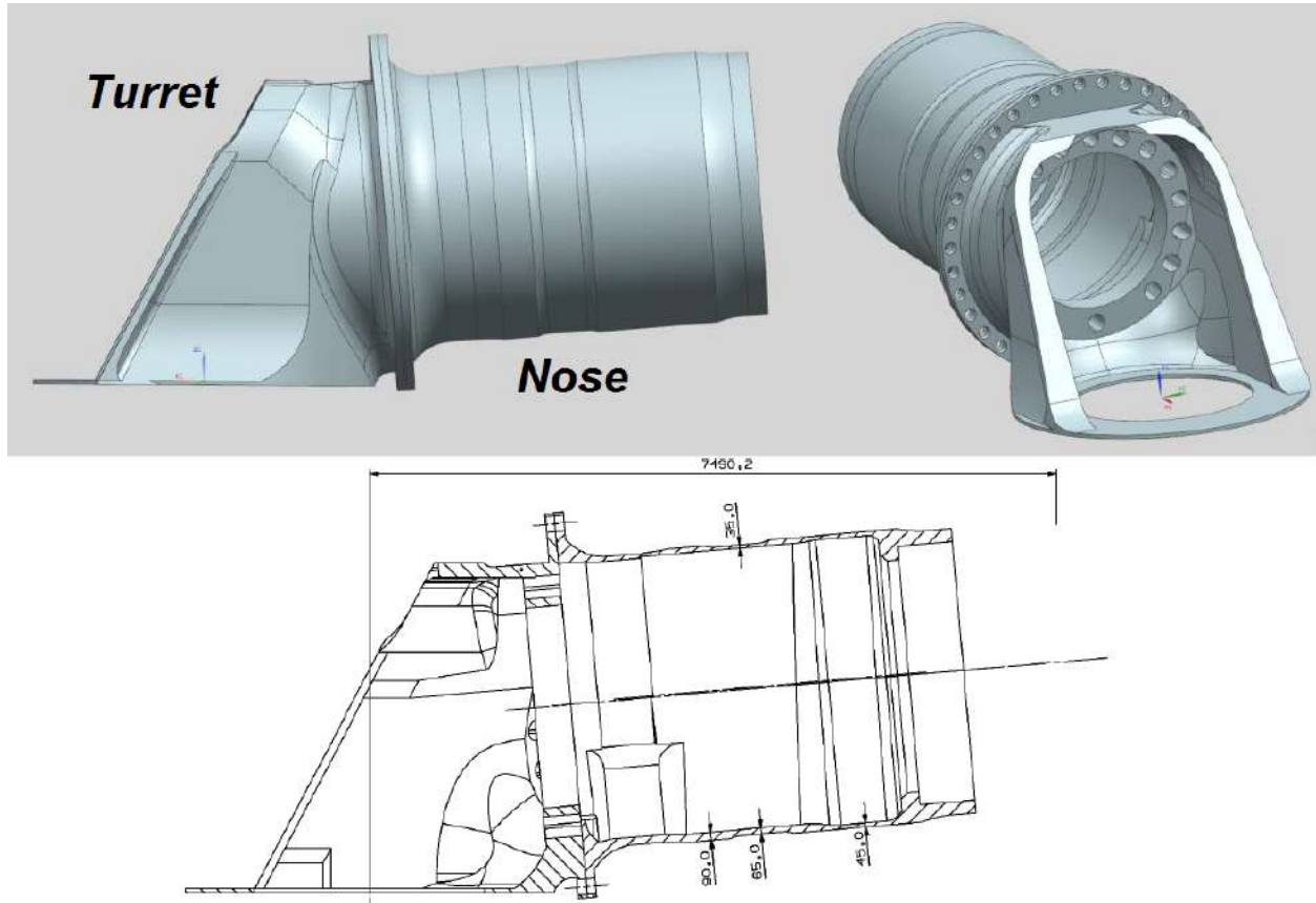
Figure 27: A CAD illustration of the bedplate.
