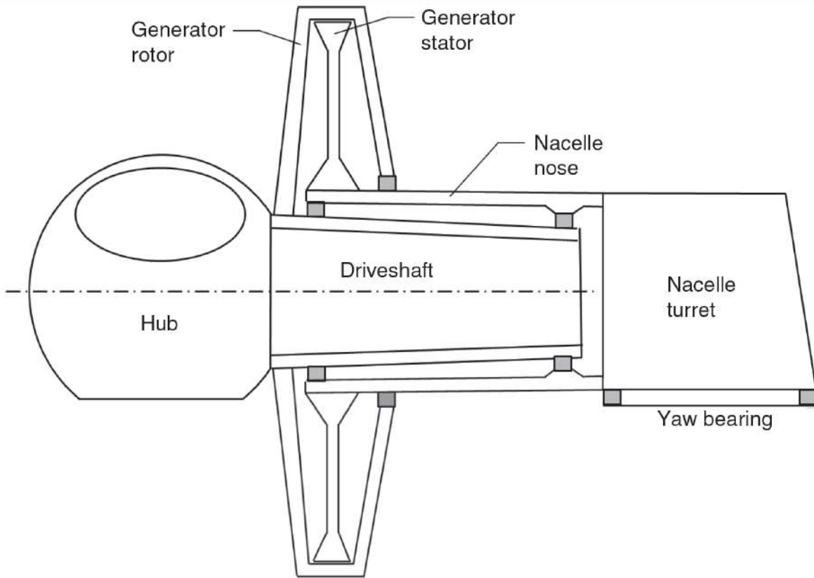
Figure 26: A sketch of the nacelle layout of the 10-MW direct-drive wind turbine, not to scale with structural details omitted. Blades (not shown), hub, shaft, and generator rotor rotate. Bearings are shaded grey.
