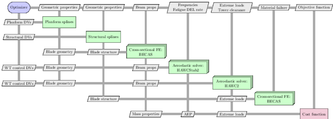
Figure 5: Extended design structure matrix diagram of the workflow of HAWTOpt2.
