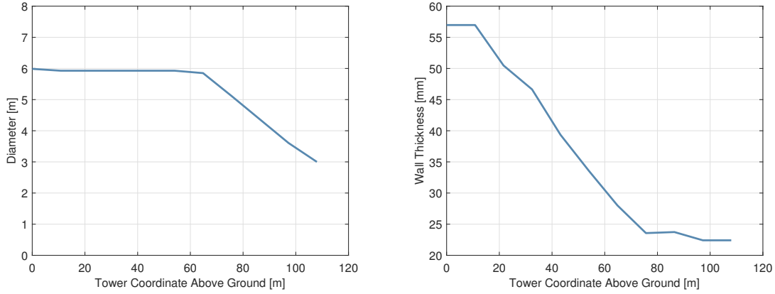
Figure 15: Structural design of the tower for the land-based wind turbine.
