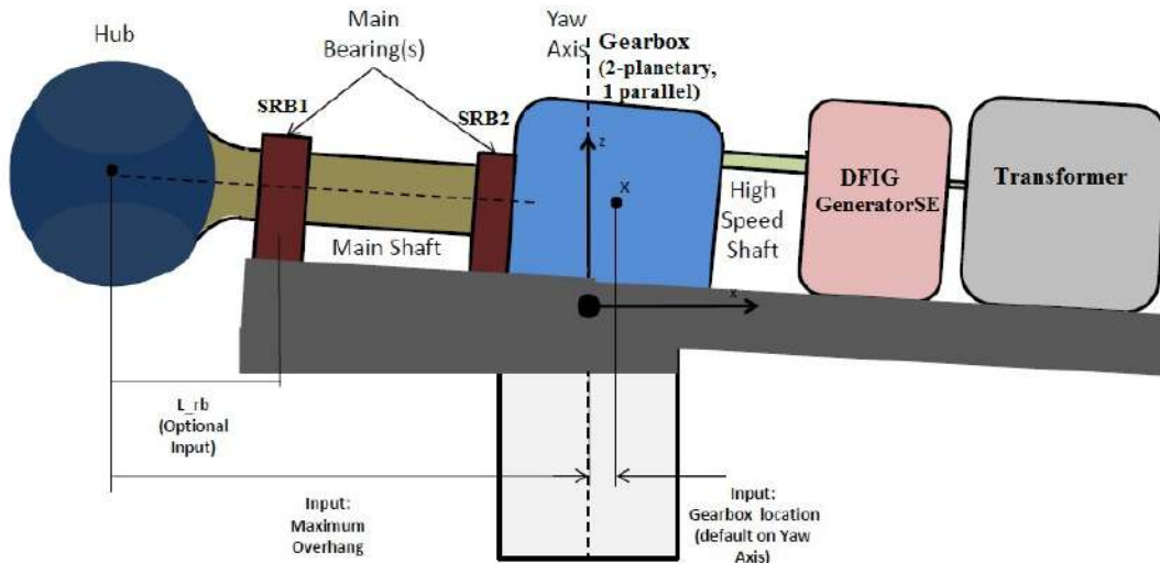
Figure 13: Drivetrain layout.
