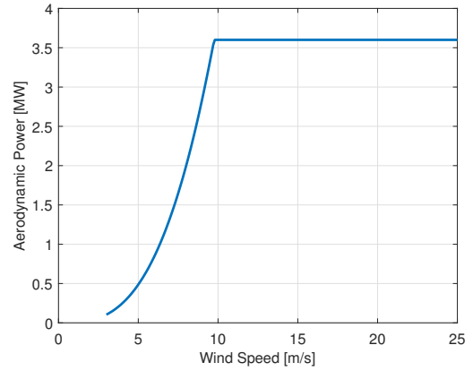
(f) Aerodynamic power
