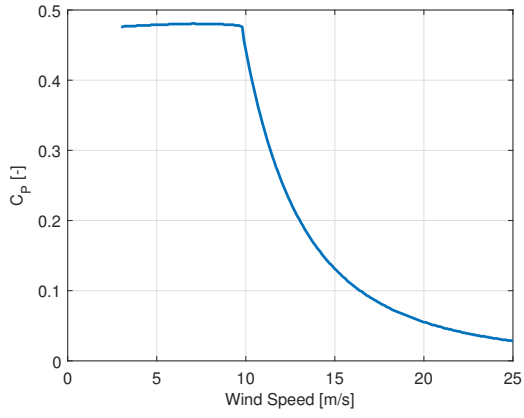
(a) Power coefficient
