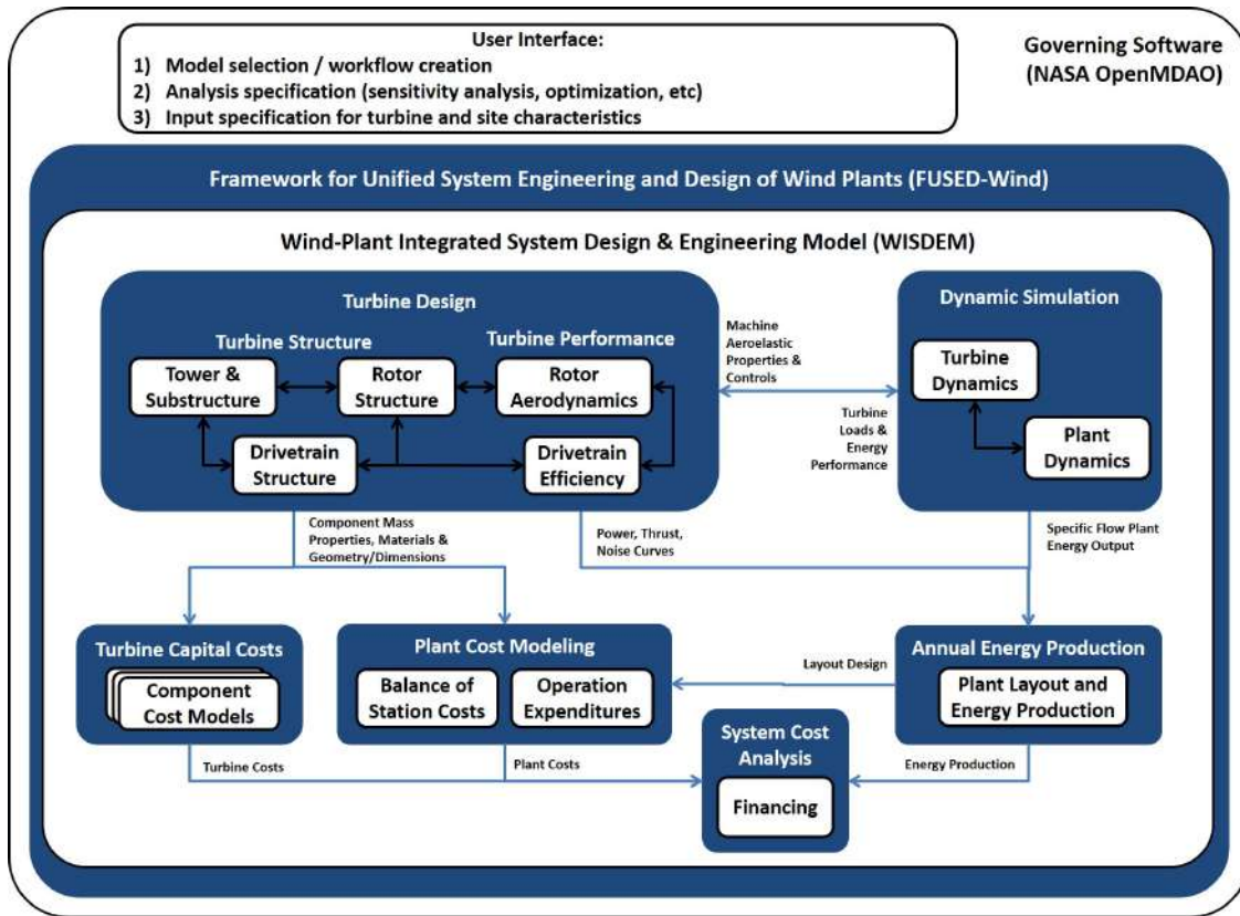
Figure 6: The Wind-Plant Integrated System Design and Engineering Model.
