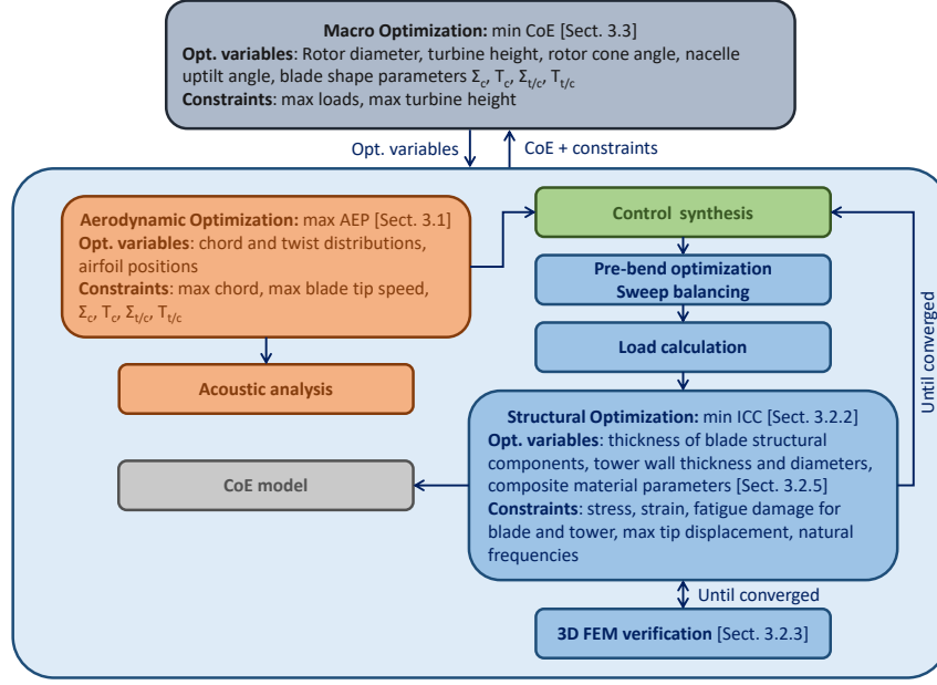
Figure 4: Algorithmic structure of Cp-Max.
