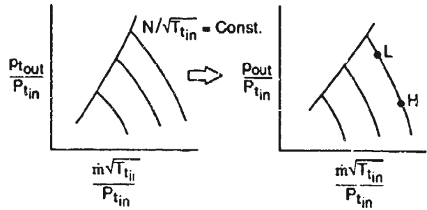
Figure 6: Parallel compressor model for high speed compressors.
