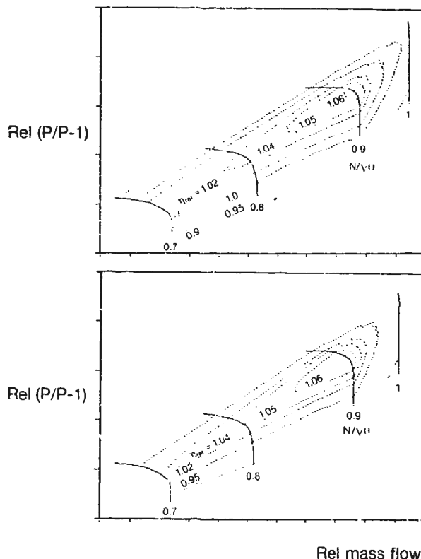
Fig. 6: Effect of 1° Restagger of the First Rotor on the Compressor Characteristic
