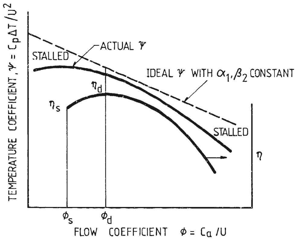
FIG. 5 STAGE CHARACTERISTIC.
