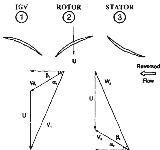
Figure 32 Mean Radius Section of a Compressor Stage in Reversed-Flow Operation.
