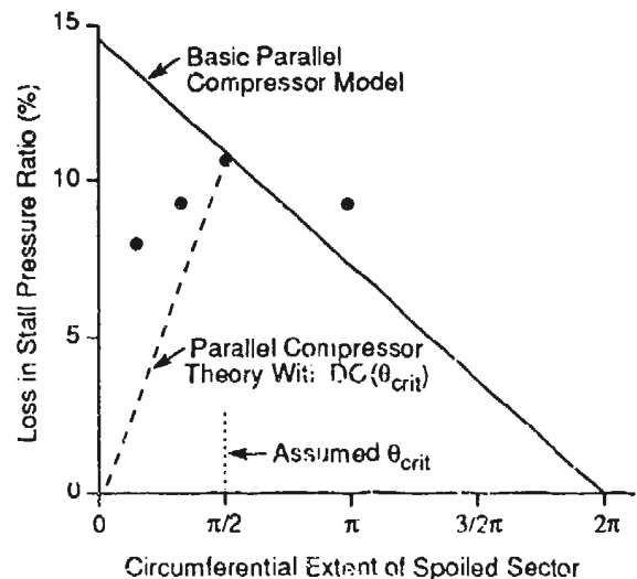
Figure 11: Prediction of loss in surge margin using parallel compressor analysis plus DC(\theta_{crit}) concept [10].
