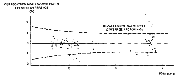
FIGURE 18 - MEASUREMENT - REPRODUCTION COMPARISON - FAN EXIT PRESSURE P23A
