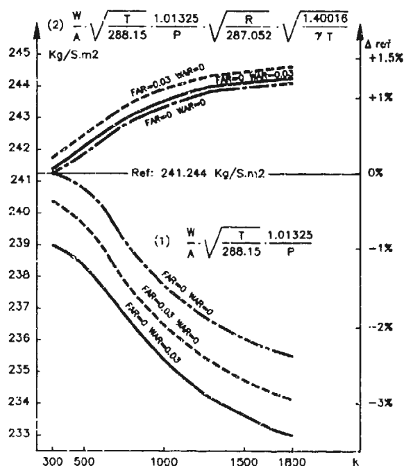
FIGURE 7 - VARIATIONS OF THE CORRECTED MASS FLOW (1) (2) WITH
