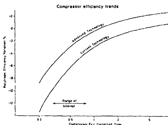
FIG.38 COMPRESSOR SIZE EFFECT (FROM REF 22)
