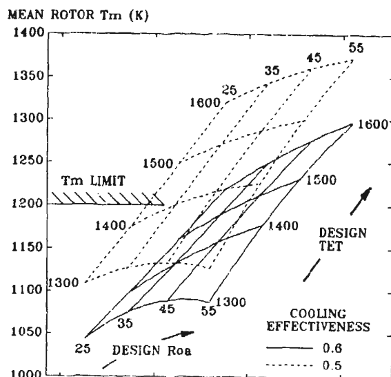
FIG. 16 HP TURBINE ROTOR METAL TEMPERATURES AT HDTO
