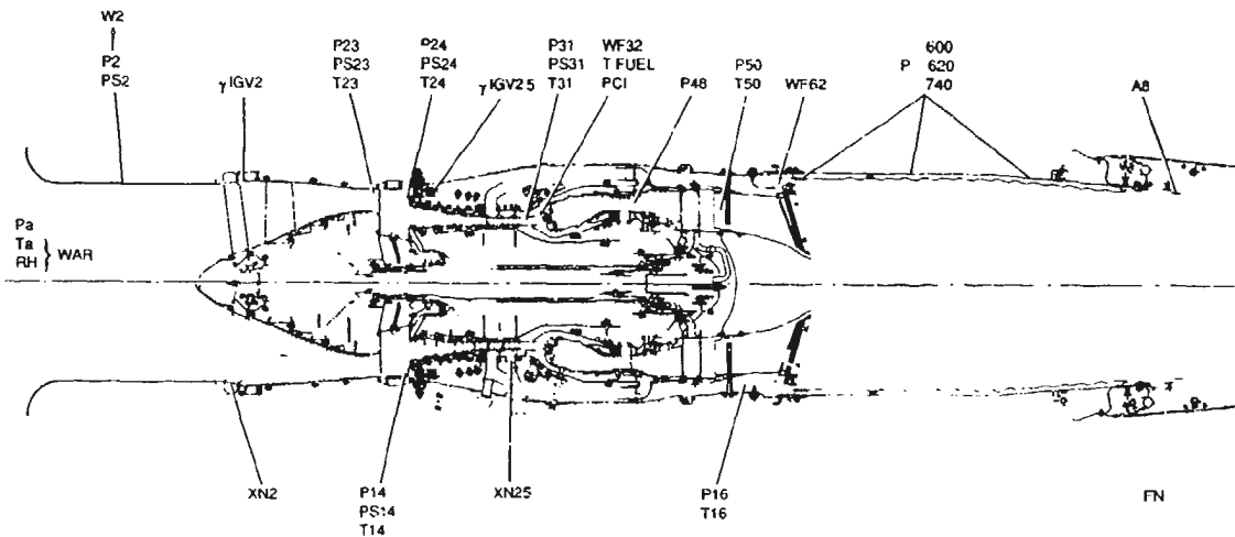
FIGURE 9 - LOCATION OF FLOW PATH MEASUREMENTS ON M88-2 ENGINE
