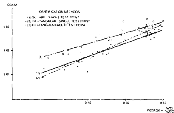
FIGURE 12 FAN FLOW CORRECTION FACTOR
