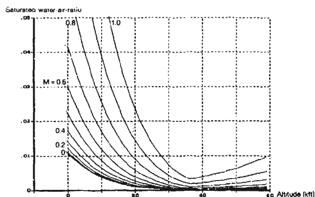
Fig. 8: Water-Air-Ratio for Saturated Conditions during ATF Tests as Function of Altitude and Simulated Flight Mach Number
