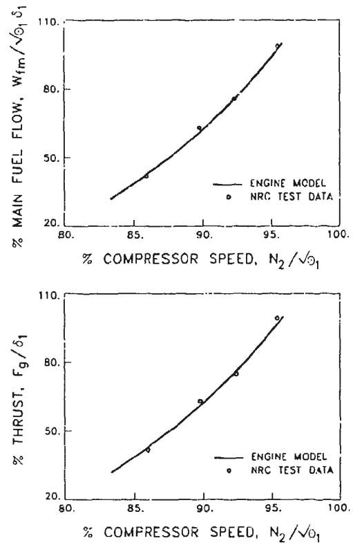
Figure 18 Steady State Performance of F404-GE-4C Engine
