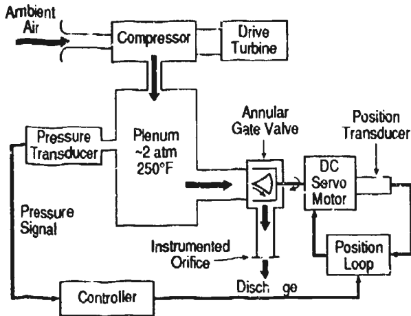
Fig. 4: Experimental setup of actively stabilized centrifugal compressor [10].
