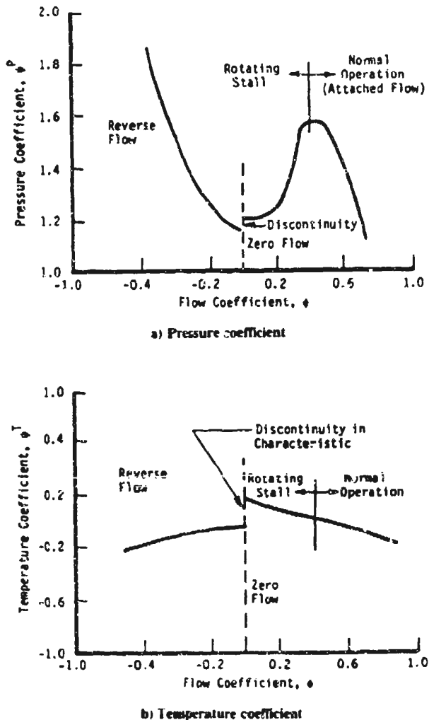
Figure 2 Typical Stage Characteristics.
