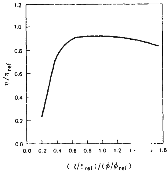
Figure 6 Generalized Stage Efficiency Characteristic
