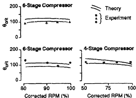
Figure 27: Predicted and experimental critical sector angles [10].
