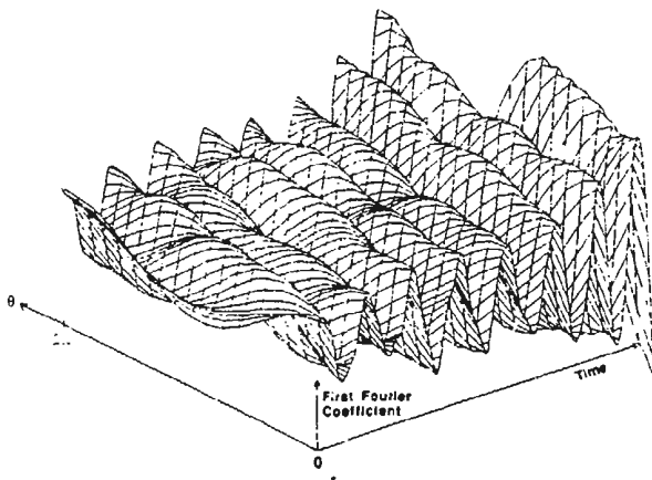
Fig. 18: Measured first harmonic behavior at stall onset [19].
