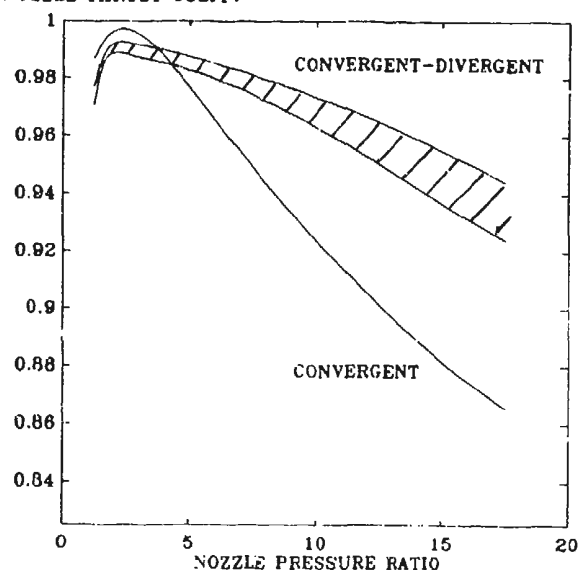
FIG.11 CONVERGENT AND CONVERGENT-DIVERGENT NOZZLES
