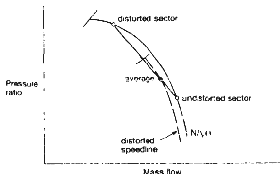
Fig. 16: Compressor Operating Points from Parallel Compressor Theory
