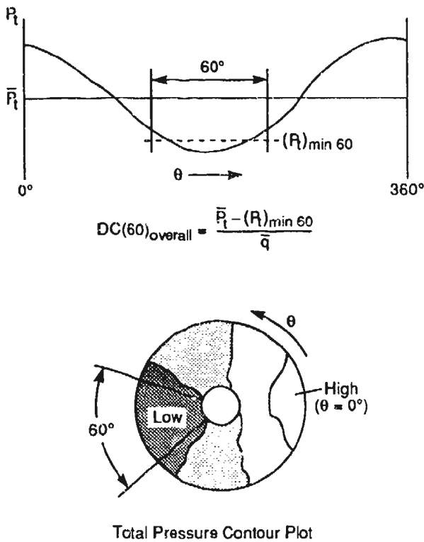
Figure 10: Definition of DC(\theta_{crit}) parameter for inlet total pressure distortion [10].
