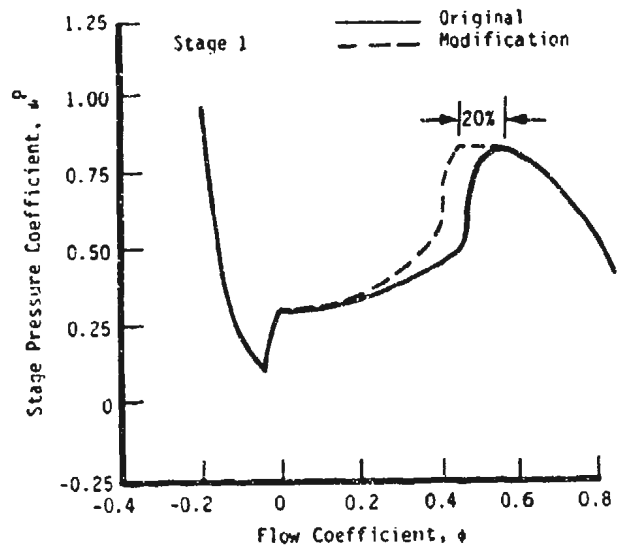
Figure 15 Postulated Stage Pressure Characteristic Modification as a Result of Tip Treatment.
