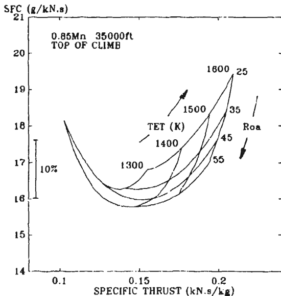
FIG.12 AERODYNAMIC DESIGN POINTS - CIVIL ENGINES
