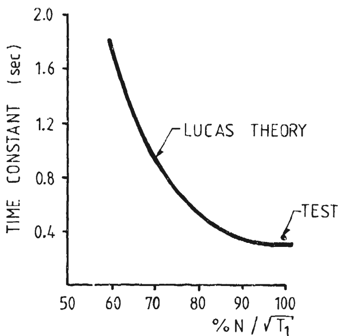
FIG. 12 VARIATION OF TIME CONSTANT WITH SPEED
