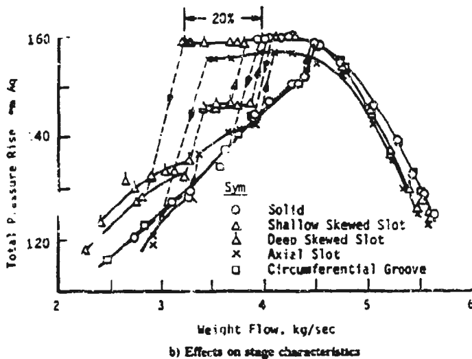
Figure 14 Possible Tip Treatment Modification and Its Effect on Stage Characteristics.
