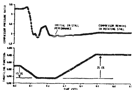
Figure 22 Model Simulation of Experimentally-Determined Compressor Recovery Hysteresis.
