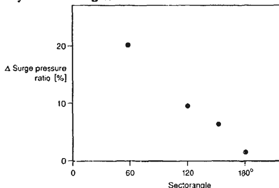
Fig. 18: Dynamic Surpline Shift Analyzed from Rig Tests
