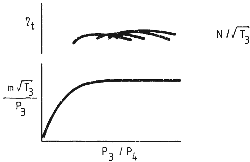
FIG. 6 TURBINE CHARACTERISTIC
