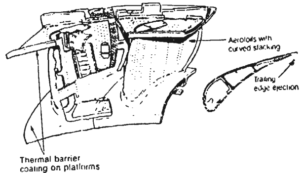
FIG.7 RB211535E4 NOZZLE GUIDE VANE (FROM REF 6)
