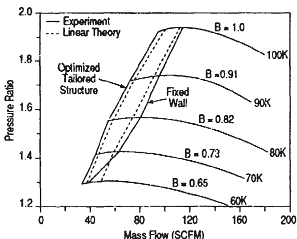
Fig. 13: Predicted and measured stability limits with dynamic structural control [11].
