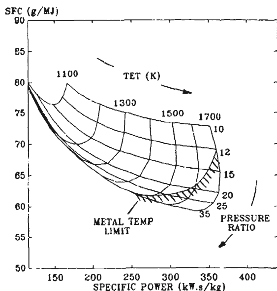
FIG.37 BASIC SHAFT POWER ENGINE PERFORMANCE
