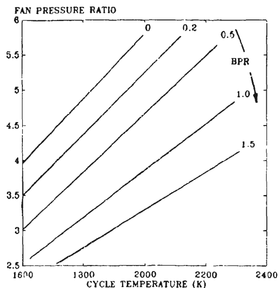
FIG. 28 FAN PRESSURE RATIO/BYPASS RATIO RELATIONSHIP MILITARY TURBOFAN
