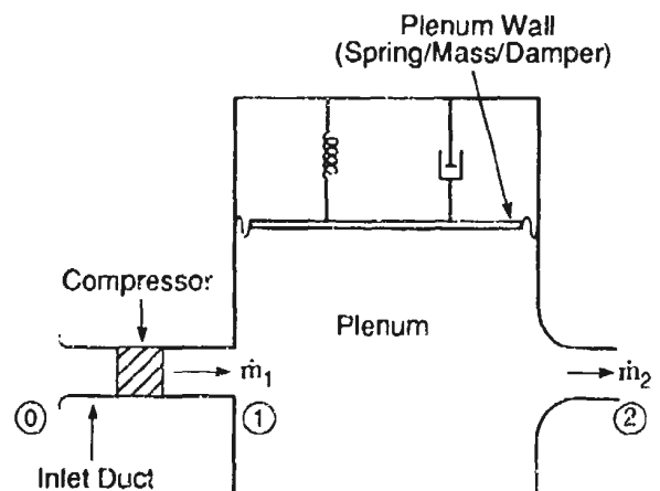
Fig. 9: Schematic of moveable plenum wall compression system [11].
