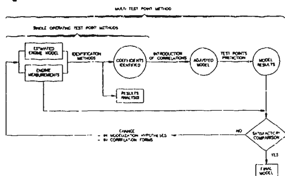
FIGURE 11 - TEST PROCESSING DIAGRAM
