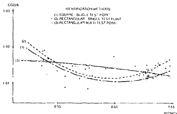
FIGURE 13 FAN EFFICIENCY CORRECTION FACTOR
