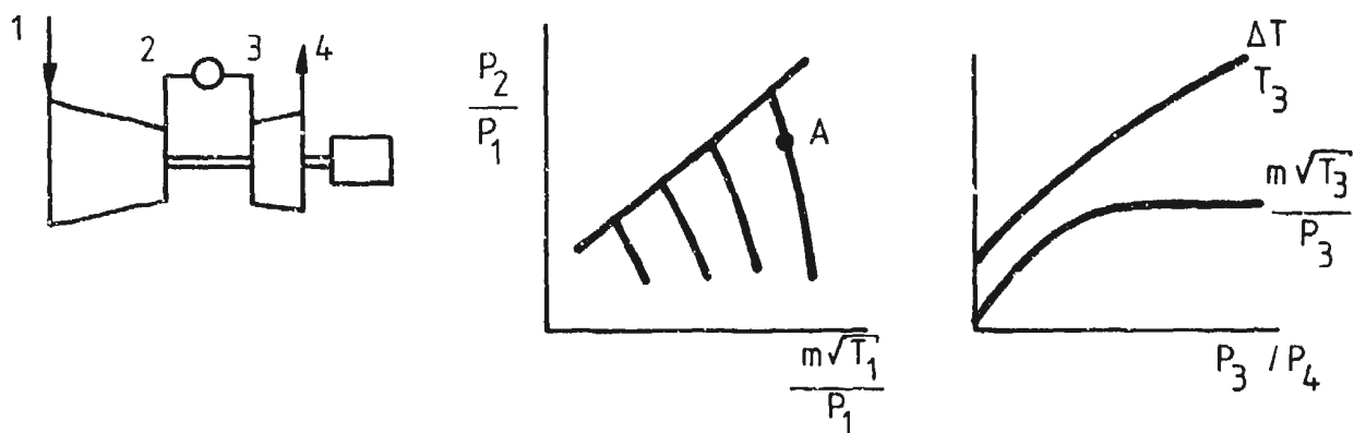
FIG. 7 SINGLE SHAFT
