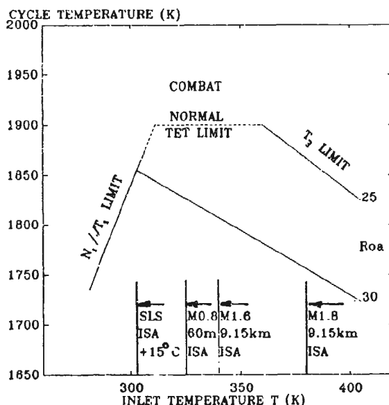
FIG. 31 MILITARY TURBOFAN - TYPICAL RATING DIAGRAM
