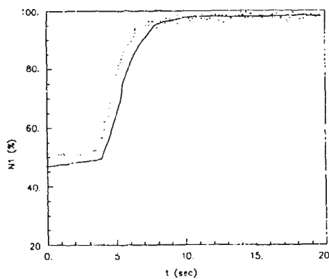
Figure 19-a Comparison of Model Fan Speed Performance with Flight Data
