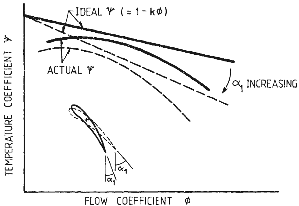
FIG.7 EFFECT OF VARIABLE STATORS
