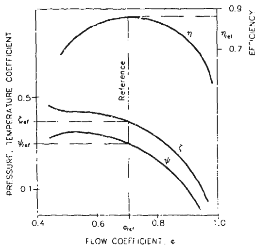
Figure 4 Compressor Stage Characteristics
