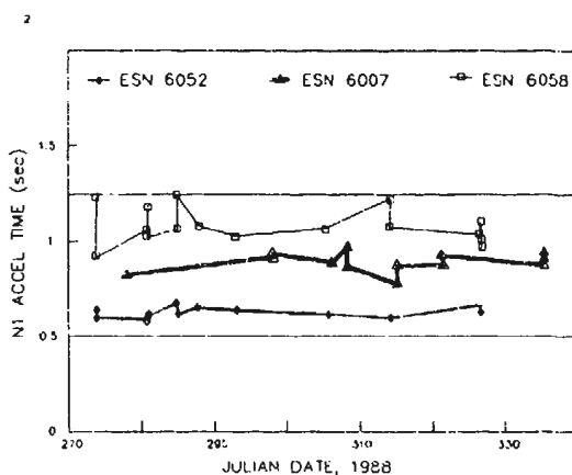
Figure 25 Trend Plots of Different F404-GE-400 Engines
