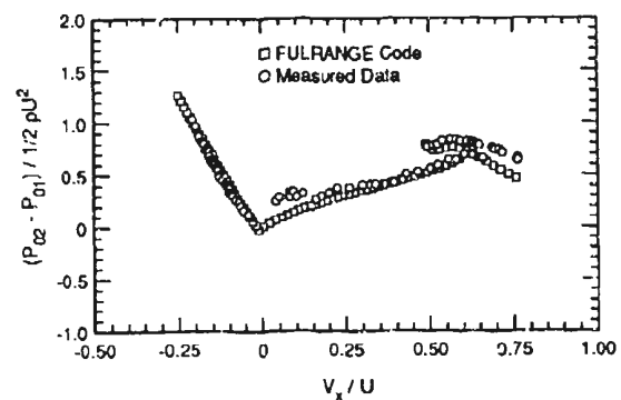
Figure 34 Three-Stage Test Compressor First Stage Pressure Characteristic.
