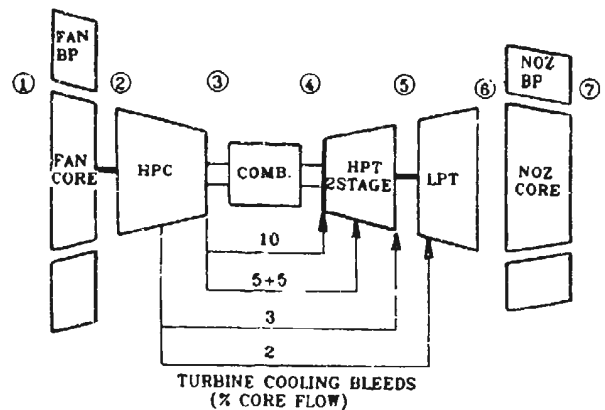
FIG.3 ENGINE CYCLE DIAGRAM (CIVIL TURBOFAN)
