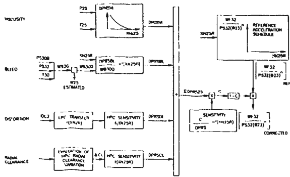
FIGURE 22 - M88-2 ADAPTIVE ACCELERATION SCHEDULE
