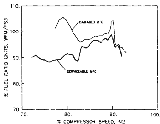
Figure 30 Transient Record of Damaged Main Fuel Control
