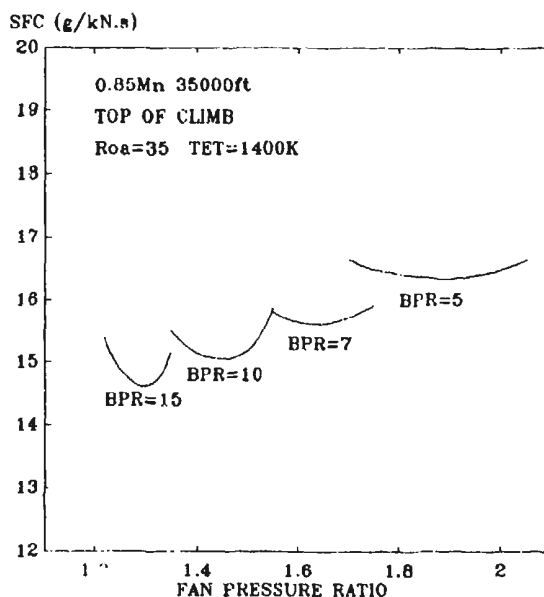
FIG.19 AERO DESIGN POINTS - FPR OPTIMISATION
