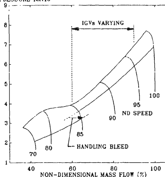
FIG.2 TYPICAL MILITARY HP COMPRESSOR CHARACTERISTIC
