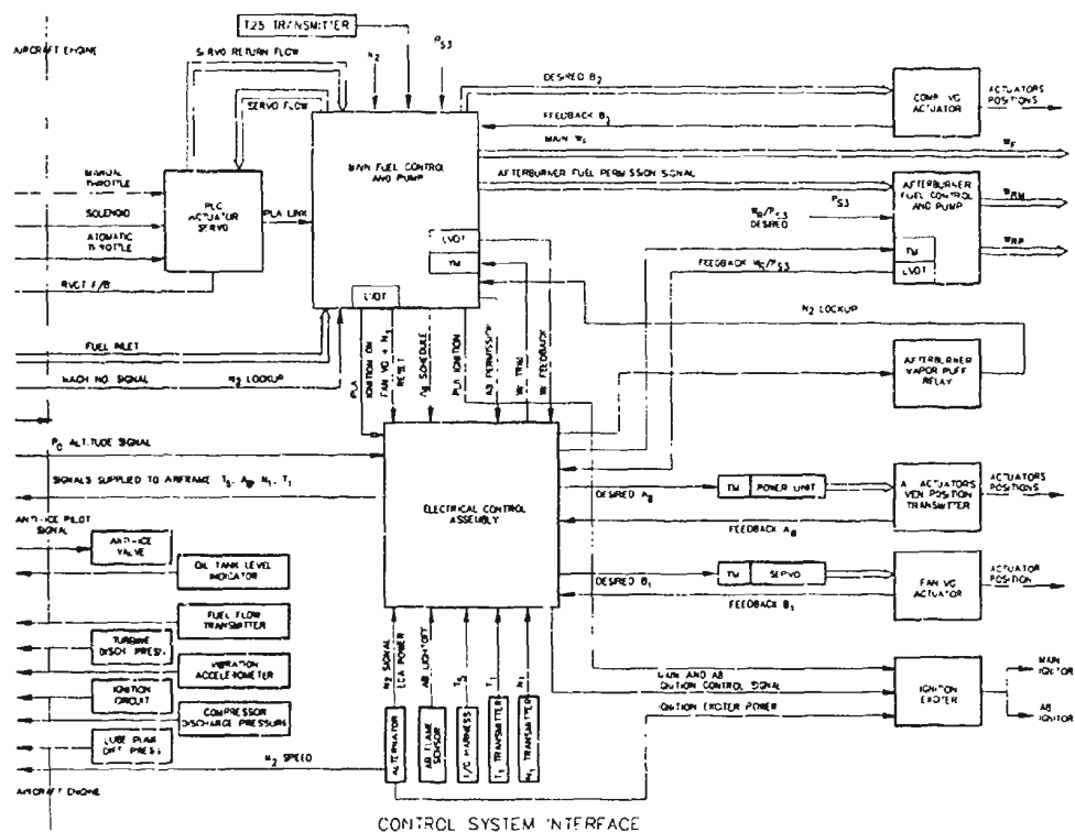
Figure 10 Overall Control System Structure
