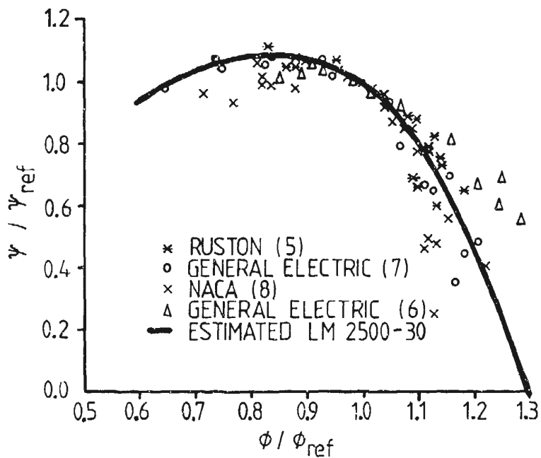
FIG.8 GENERALIZED STAGE PRESSURE COEFFICIENT CURVE (FROM REF 8)
