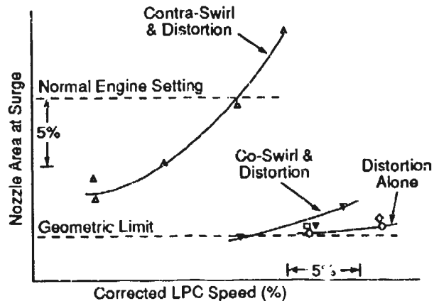
Figure 14: Effect of inlet swirl and total pressure distortion on compressor instability [10].
