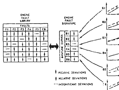
Figure 27 Fault Diagnostic Procedure
