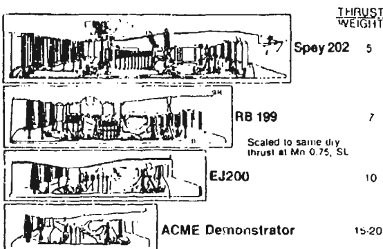
FIG.35 ENGINE THRUST/WEIGHT RATIO TRENDS (FROM REF 18)
