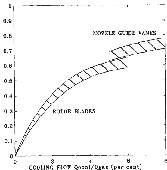
FIG. 9 TYPICAL BLADE COOLING EFFECTIVENESS TREND
