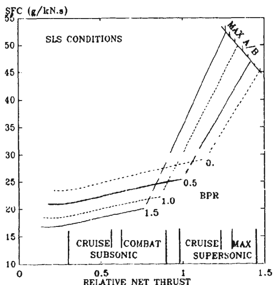
FIG. 30 MILITARY ENGINE PERFORMANCE - EFFECT OF BYPASS RATIO
