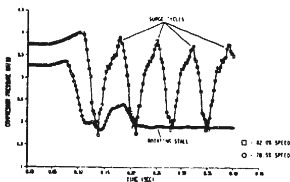
Figure 19 Model Simulation of Experimentally-Determined Rotating Stall/Surge Boundary.
