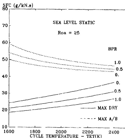
FIG. 29 MILITARY ENGINE SFC TRENDS
