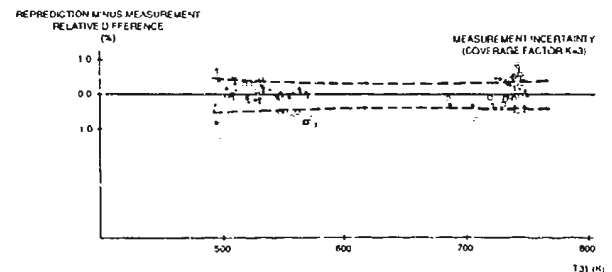
FIGURE 19 - MEASUREMENT - REPRODUCTION COMPARISON - HPC EXIT TEMPERATURE T31
