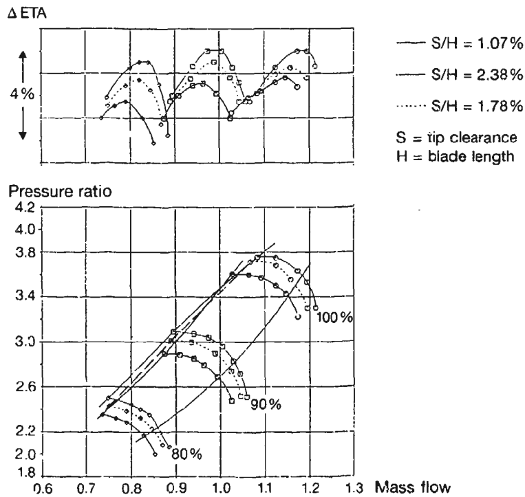
Fig. 3: Effects of Tip Clearance on Compressor Characteristics
