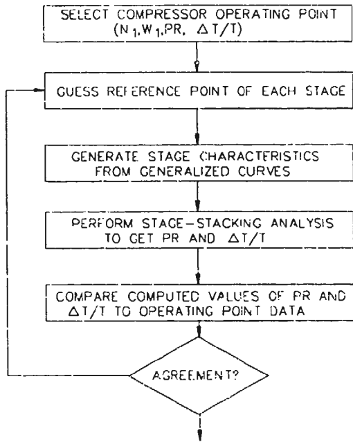
Figure 7 Flowchart for Compressor Characteristic Development
