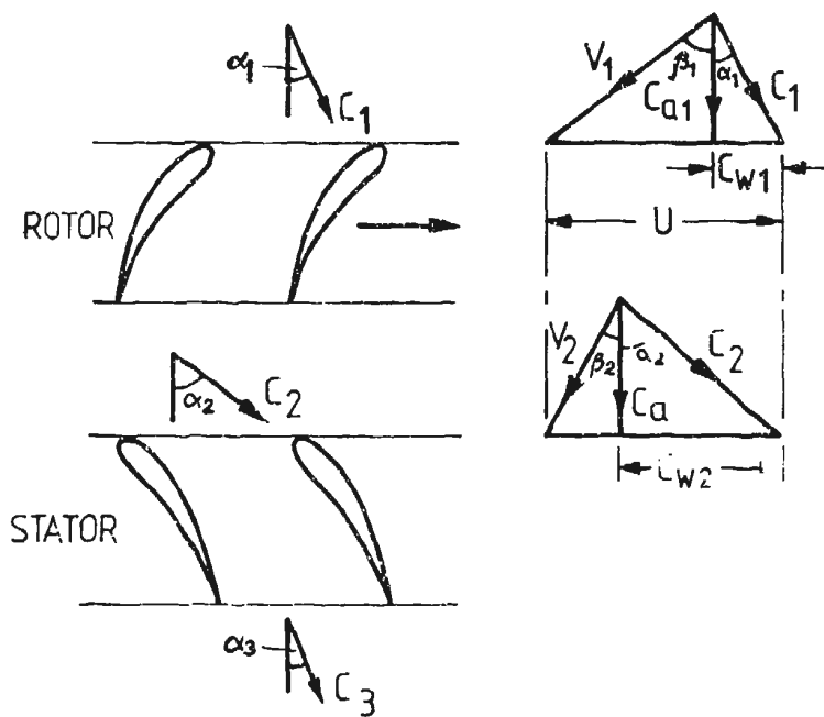
FIG. 4 VELOCITY TRIANGLES (AXIAL FLOW COMPRESSOR)
