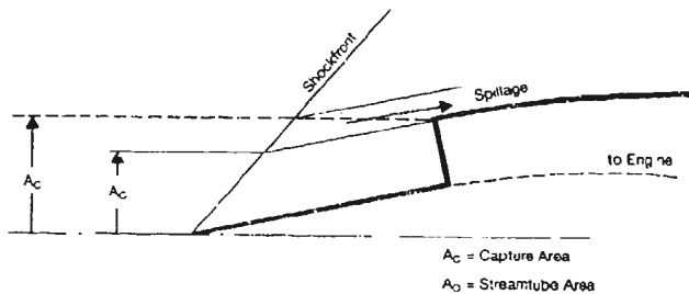
Fig. 24: Spillage Around an Intake
