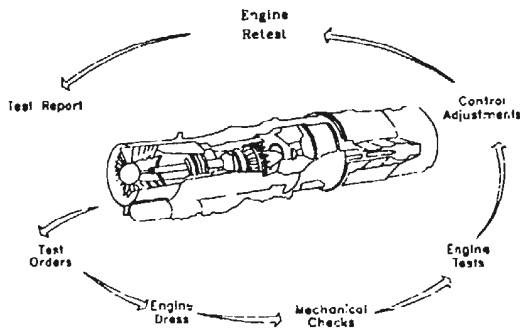
Figure 1-c Engine Test Environment
