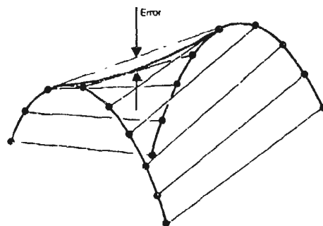
Fig. 13: Linear Interpolation Error
