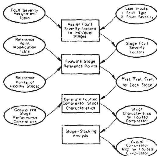
Figure 1: Axial Compressor Fault Modelling
