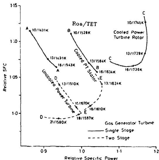
FIG. 40 SMALL TURBOSHAFT ENGINE PERFORMANCE (FROM REF 22)
