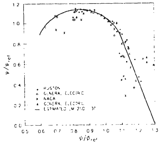
Figure 5 Generalized Stage Pressure Rise Coefficient
