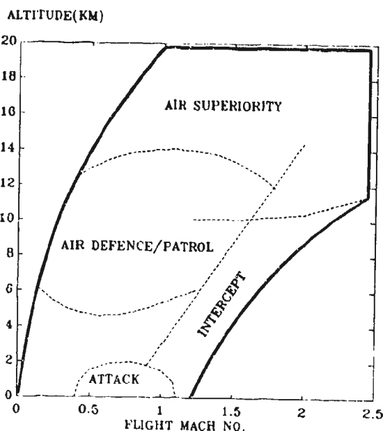
FIG. 24 MILITARY AIRCRAFT FLIGHT ENVELOPE
