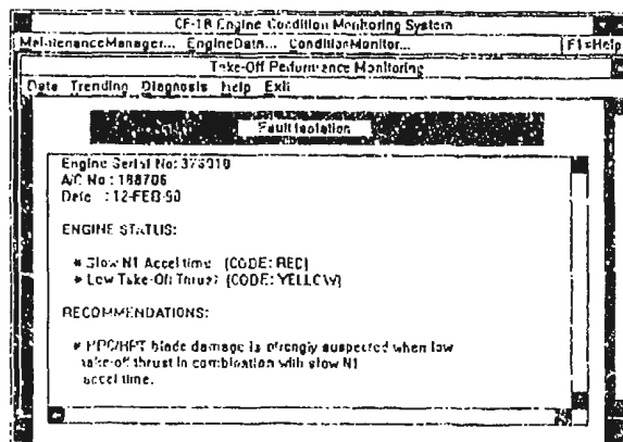
Figure 28-b Typical Diagnosis Provided to Operator
