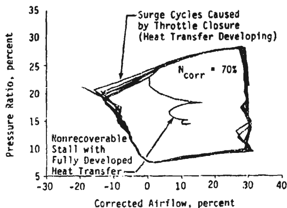
Figure 13 Effect of Compressor Heat Transfer (blade to gas path) on Poststall Behavior, Nine-Stage HPC at 70% Speed.
