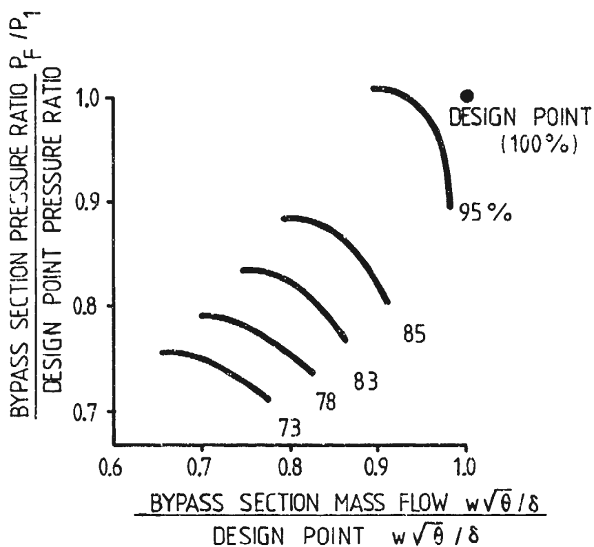
FIG. 1 SINGLE STAGE FAN CHARACTERISTIC (FROM REF.1)
