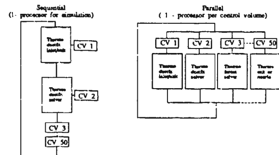
Figure 41 Comparison Between Serial and Parallel Computational Approaches.
