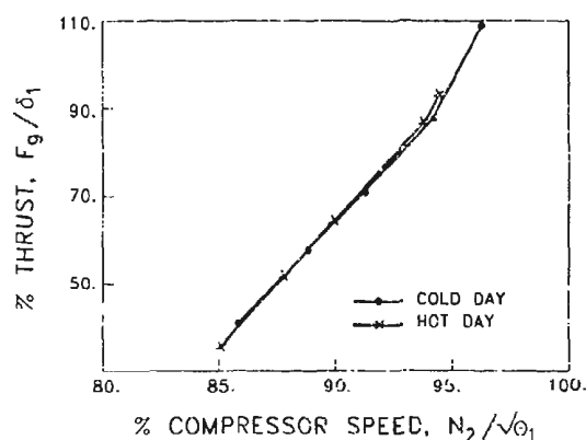
Figure 26 The Effect of Choice of Engine Baseline Parameter on Data Scatter
