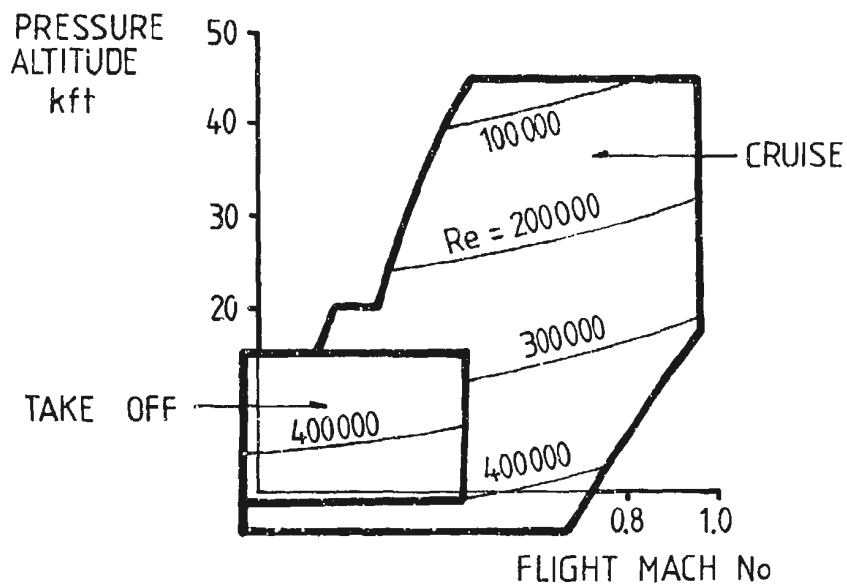
FIG. 3 REYNOLDS NUMBER VARIATION, LP TURBINE (FROM REF. 5)
