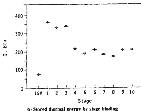
Figure 10 Predicted Stage Temperature Distribution at Maximum and Idle Power and Corresponding Blade Stored Thermal Energy in Each Stage.
