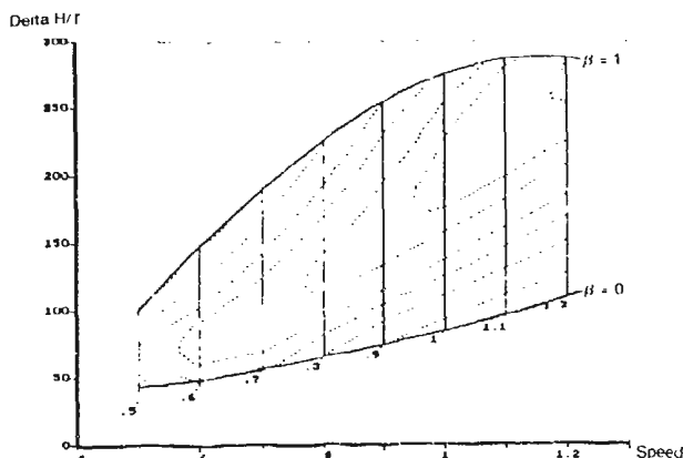
Fig. 12: Example for a Turbine Map
