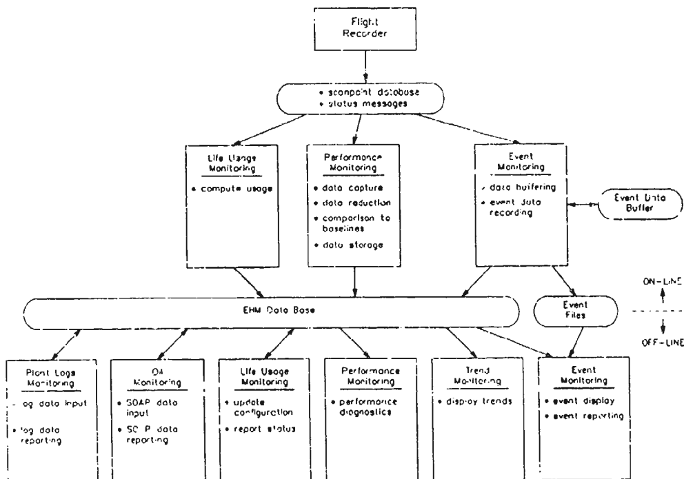
Figure 2 Overview of EHM System
