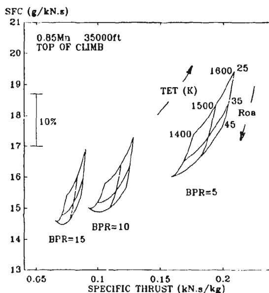
FIG.18 AERO DESIGN POINTS - EFFECT OF BYPASS RATIO
