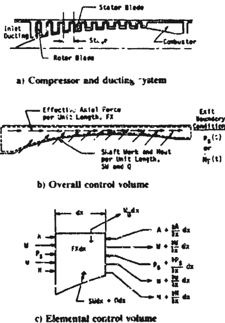
Figure 1 Physical Compression System and Control Volume Concepts.
