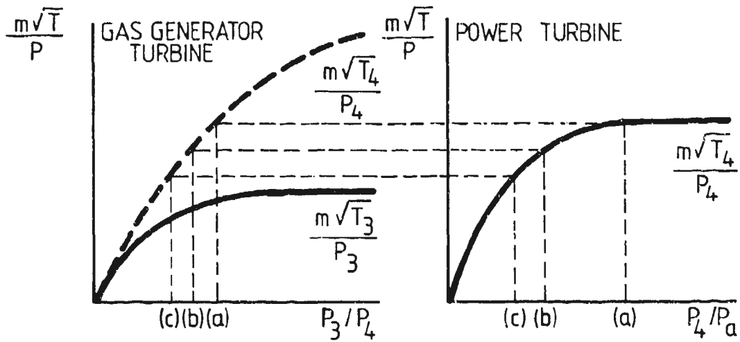
FIG. 9 OPERATION OF TURBINES IN SERIES
