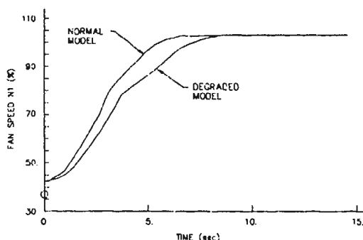
Figure 21 Model Prediction of Engine Dynamic Performance with Damaged HP Turbine
