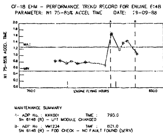
Figure 29 Typical Trend Plot of Health Index
