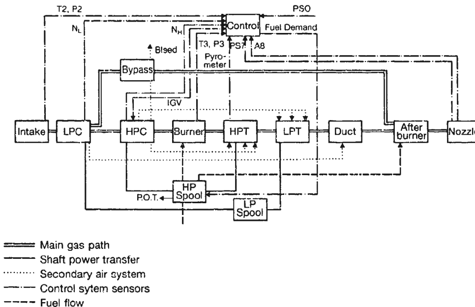
Fig. 22: Modular Performance Synthesis Structure for a Mixed Flo / Turbofan
