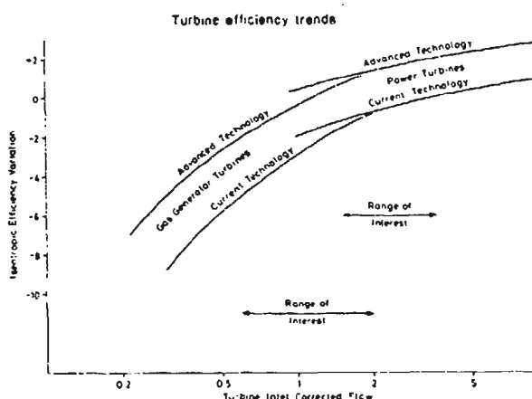
FIG.39 TURBINE SIZE EFFECT (FROM REF 22)
