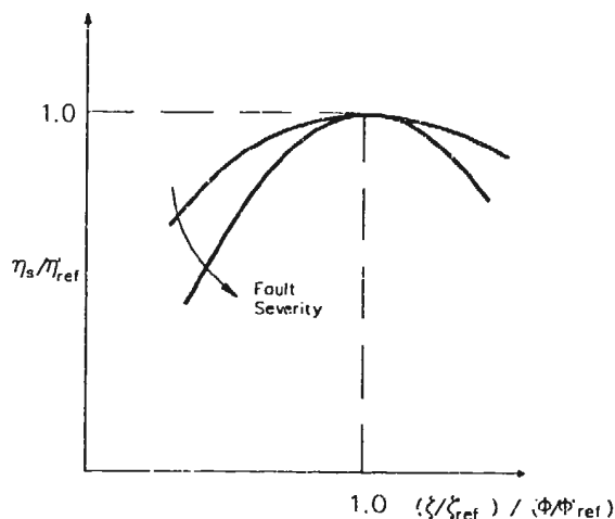
Figure 14 Typical Variation in Stage Efficiency due to Degradation
