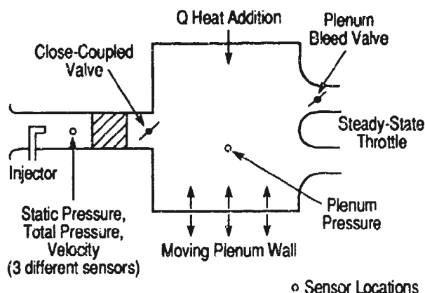
Fig. 14: Schematic of actuators and sensors evaluated [13].
