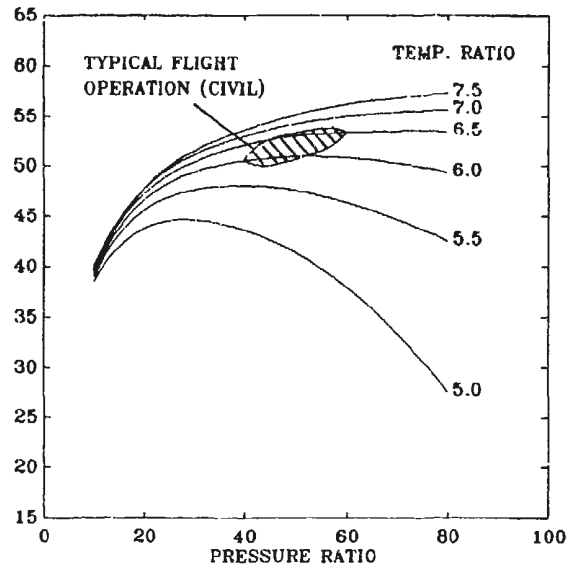
FIG.14 ENGINE THERMAL EFFICIENCY VARIATIONS
