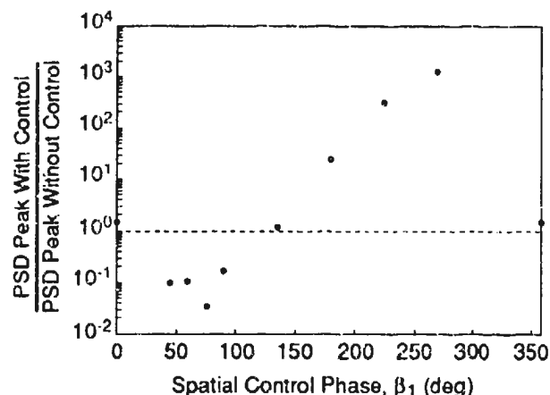
Fig. 25: Influence of feedback control phase angle ( \beta_1 ) on the strength of the first spatial mode of the flow in the compressor at \phi = 0.475 [21].
