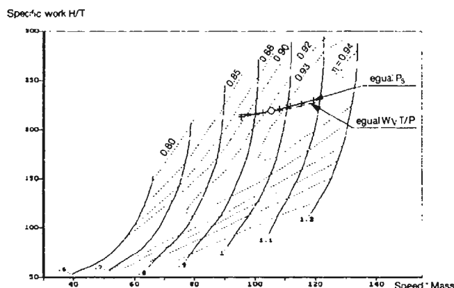
Fig. 19: Turbine Operating Points from Parallel Turbine Theory
