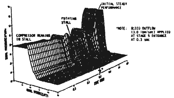
Figure 26 Stall Related Prediction Resulting From Stage 5 Bleed Outflow.
