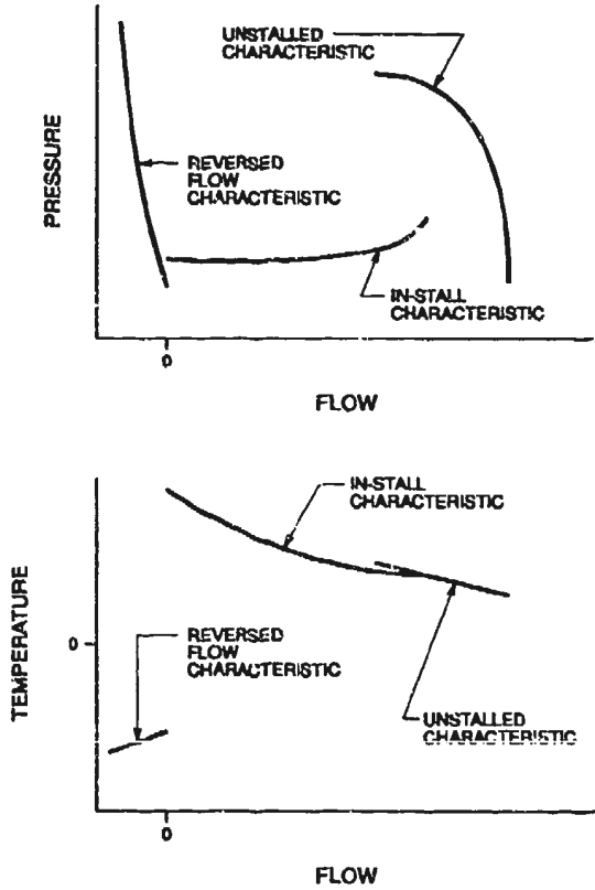
Figure 29 Full-Range Compressor Stage Characteristic.
