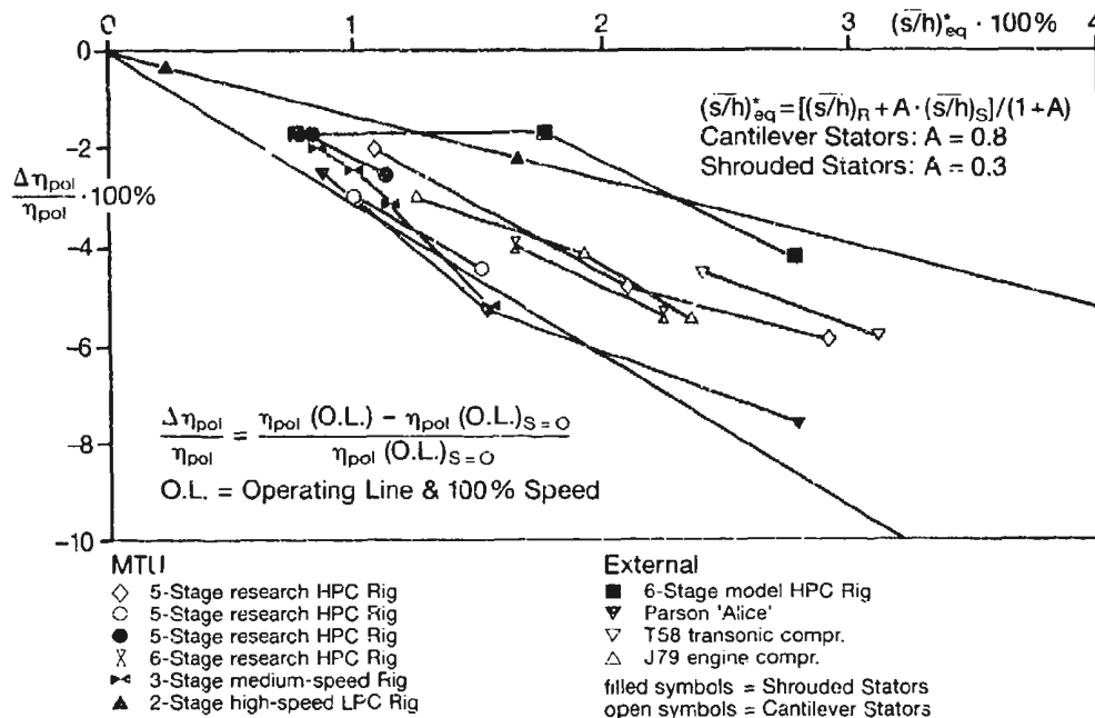
Fig. 1: Efficiency Loss in Multistage Axial Flow Compressors Due to Tip Clearance
