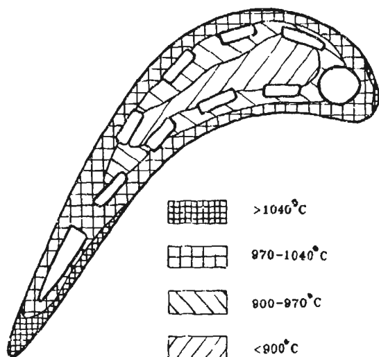
FIG. 8 TEMPERATURE VARIATIONS IN TURBINE ROTOR AIRFOIL
