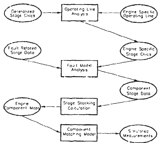
Figure 3 Overall Modelling Concept
