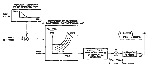
FIGURE 20 - M88-2 EXHAUST NOZZLE CONTROL THROUGH FAN SURGE MARGIN SET POINT
