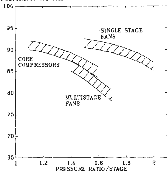
FIG.1 COMPRESSOR EFFICIENCIES - EFFECTS OF LOADING
