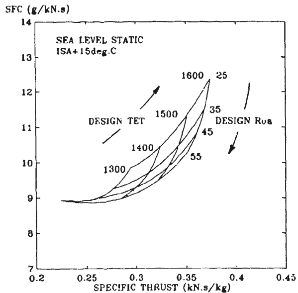
FIG.13 HDTO OFF-DESIGN POINTS - CIVIL ENGINES
