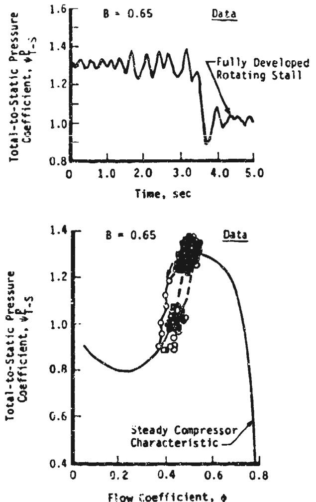
Figure 4 Poststall Behavior of Compressor Rig: Rotating Stall, B = 0.65
