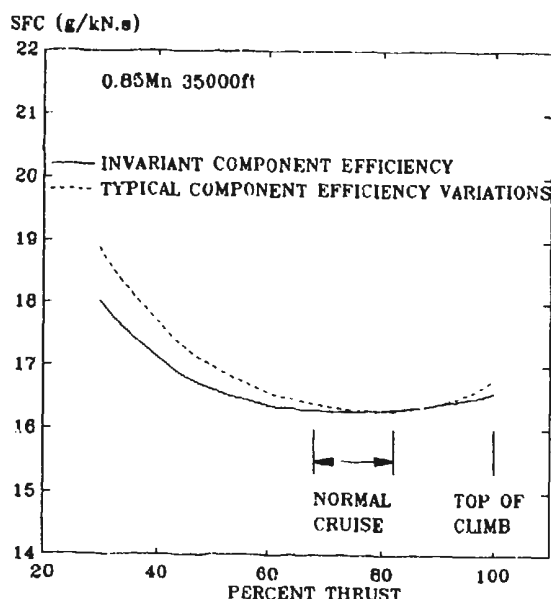
FIG.17 THRUST/SFC LOOPS FOR BPR=5 ENGINE
