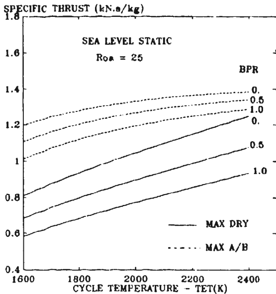
FIG. 25 MILITARY ENGINE SPECIFIC THRUST TRENDS
