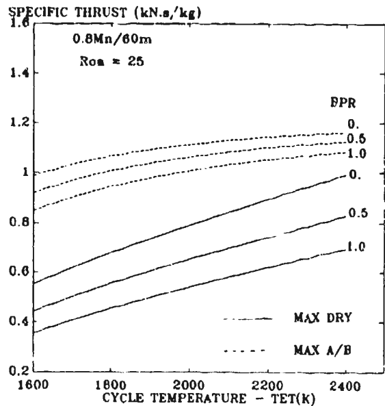
FIG. 26 MILITARY ENGINE SPECIFIC THRUST TRENDS
