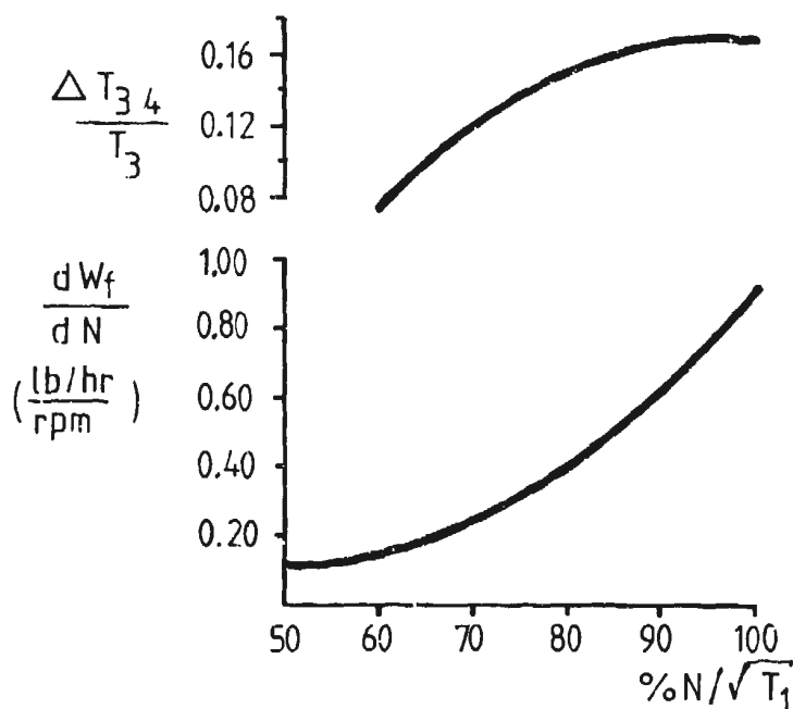
FIG. 11 PARAMETERS DETERMINING TIME CONSTANT
