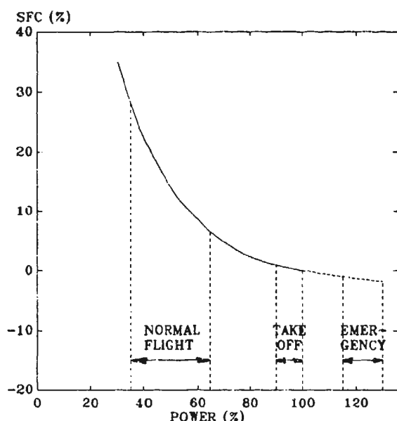
FIG. 42 TURBOHAFT ENGINE - TYPICAL SFC LOOP
