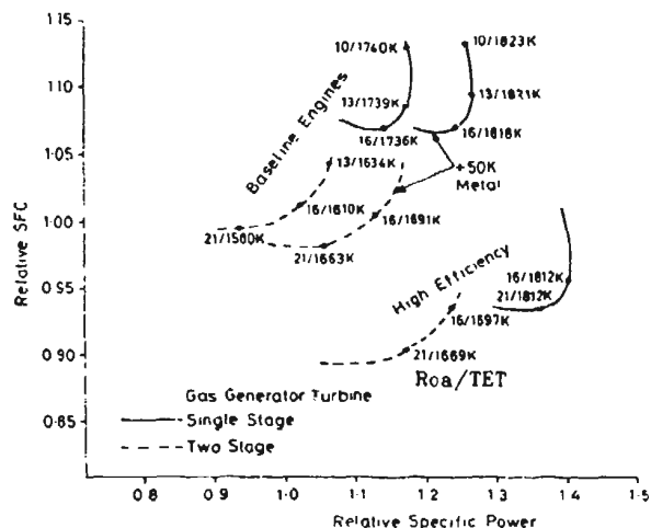
FIG. 41 SMALL TURBOSHAFT - EFFECTS OF ADVANCED TECHNOLOGY
