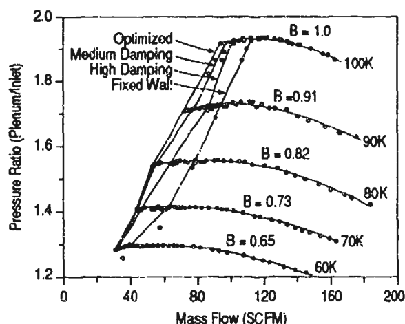
Fig. 12: Compressor map showing increase in stable flow region due to tailored structure for three values of damping; damping values \zeta = 1.5, 2.25, 3.0 , other parameters at optimized values [11].
