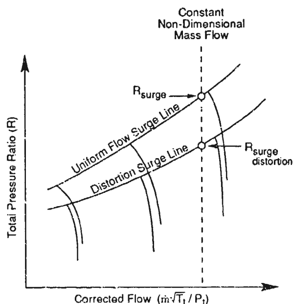
Figure 8: One definition of surge margin decrease; loss in pressure ratio at constant mass flow.
