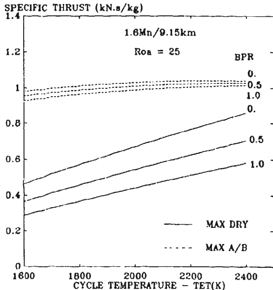
FIG. 27 MILITARY ENGINE SPECIFIC THRUST TRENDS
