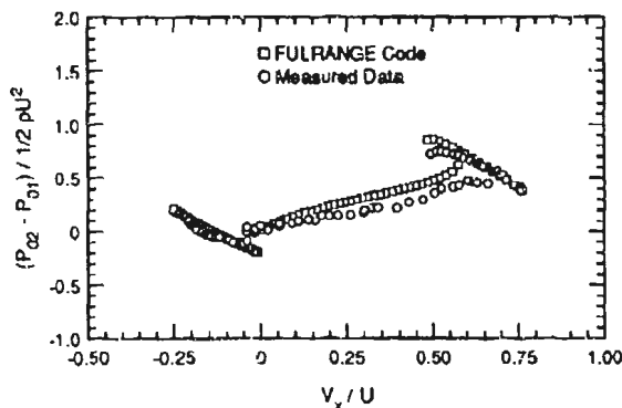
Figure 36 Three-Stage Test Compressor Third Stage Pressure Characteristic.
